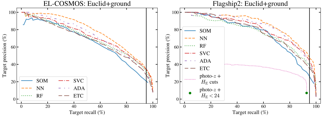
Fig. 7. Precision vs. recall curves for the analyses with Euclid photometry and ground-based photometry. Left: Results for EL-COSMOS. Right: Results for Flagship2. The dotted magenta line represents the photo- z selection for a range of H_E magnitude limits. The green marker indicates the photo- z selection with H_E < 24 .
