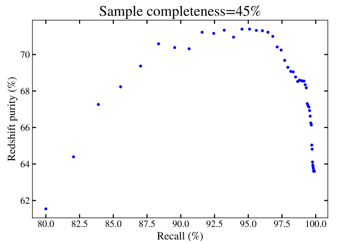
Fig. 12. Spectroscopic redshift purity and completeness with the addition of the photometric classification. Top: Curves are colour-coded as a function of the recall of the photometric classification. The spectroscopic reliability threshold varies along each curve, while varying the threshold on the photometric classification probability shifts the curve. The purity improves as recall increases, reaching a maximum for recall \sim 95\% and declining after. For better visualisation, the first lines are labelled with the corresponding recall value. At recall values above 95% the curves are tightly packed. The solid black line corresponds to 100% recall, while the dashed line to 95% recall, the value we chose to benchmark our results. Bottom: Redshift purity as a function of the recall of the photometric classification, fixing the value of sample completeness to 45%.
