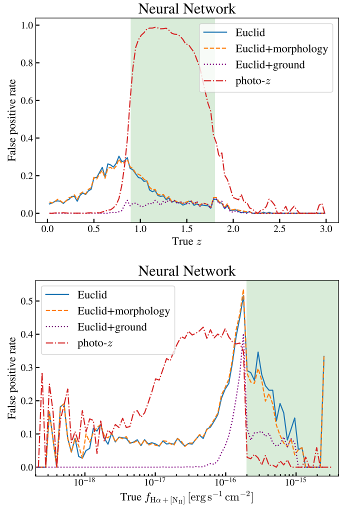
Fig. 10. False positive rate as functions of redshift and f_{\text{H}\alpha+\text{[N II]}} for Flagship2. The plot allows us to identify the origin of non-targets that enter the selected samples. The solid blue, dashed orange, and dotted purple curves, respectively, correspond to the neural networks trained with Euclid photometry, Euclid plus morphological data, and Euclid plus ground-based photometry. The dash-dotted red line is the false positive rate of the photo- z selection. Top: False positive rate as a function of z . The green shaded area marks the target redshift range. Bottom: False positive rate as a function of f_{\text{H}\alpha+\text{[N II]}} . The green shaded area corresponds to the \text{H}\alpha limiting flux. There is a peak in the false positive rate just below the flux limit used to define the target sample, although we note that these galaxies can still give correct redshift measurements.
