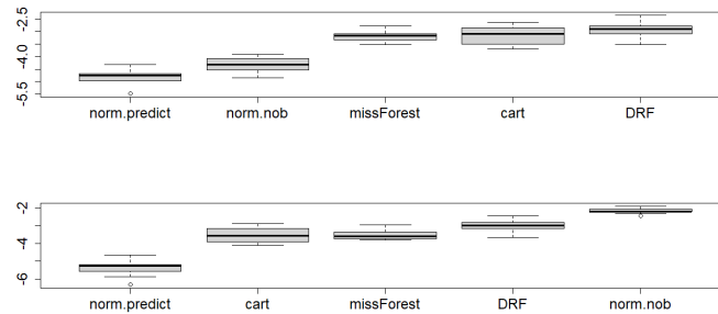
Figure 14: Scores for the nonlinear mixture model with distribution shift. Top: DRF-Score over 10 iterations. Bottom: m-I-Score over 10 iterations.
