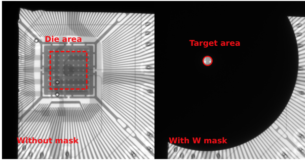
Fig. 8: X-ray snapshot of the Spartan6 chip (On the left) and an X-ray snapshot of a targeted area post W mask positioning (On the right)
