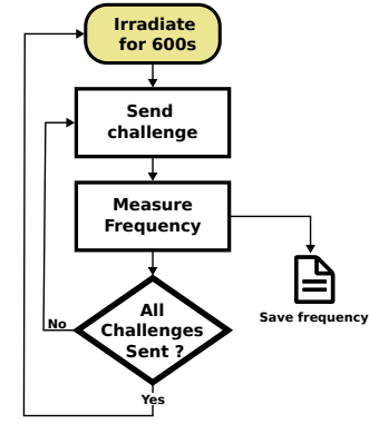
Fig. 10: Frequency measurement automation flow
