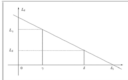
Figure 1. The graph of the straight line L_\delta
