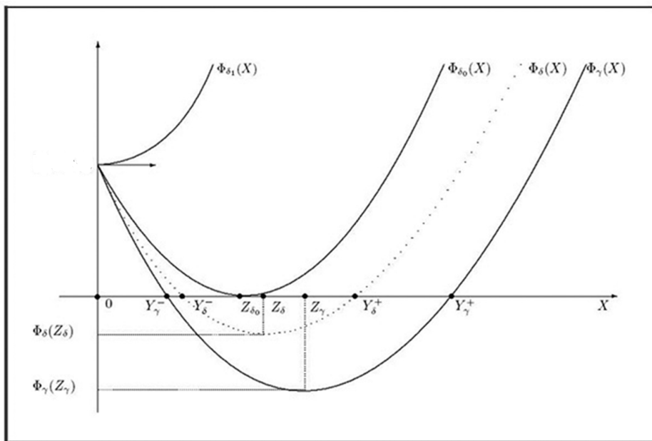
Figure 2. The graphs of the functions \Phi_\delta(X) for \delta = \gamma , \gamma < \delta < \delta_0 , \delta = \delta_0 and \delta = \delta_1
