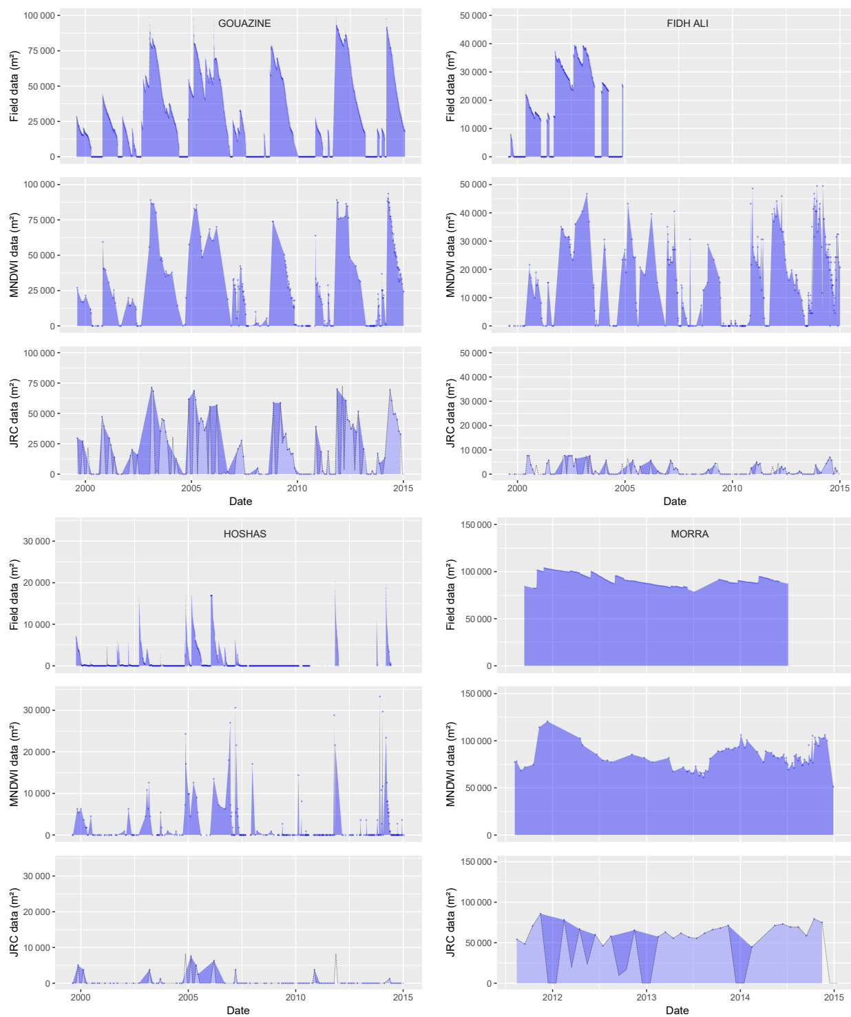
Figure 15. Surface water extent dynamics from field data and remote sensing over 1999–2015 for four lakes. JRC data (Pekel et al., 2016) are filtered to images with less than 25 % NA over the lake cell (the complete JRC datasets are represented in pale blue).
