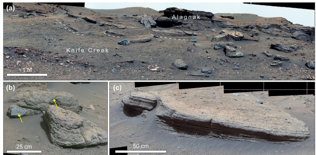
Figure 16. Alagnak member at Cape Nukshak. (a) Resistant, planar laminated sandstones ( S_1 ) and thin-bedded granule-pebble sandstones ( S_n ) of the Alagnak member within a Mastcam-Z 110 mm mosaic (zcam08613) acquired on sol 604. Dashed white lines trace the curvilinear, scoured base of several sandstone bodies. (b) Large, out-sized clasts up to 20 cm (yellow arrows) embedded within a sandstone matrix at Alagnak within a Mastcam-Z 110 mm mosaic (zcam08631) on sol 632. (c) Planar laminated sandstone ( S_1 ) within the “Hagelbargers Pass” block from the Alagnak member within a Mastcam-Z 110 mm mosaic (zcam08630) on sol 632. Grains fine upward from the base to the top of the block.
