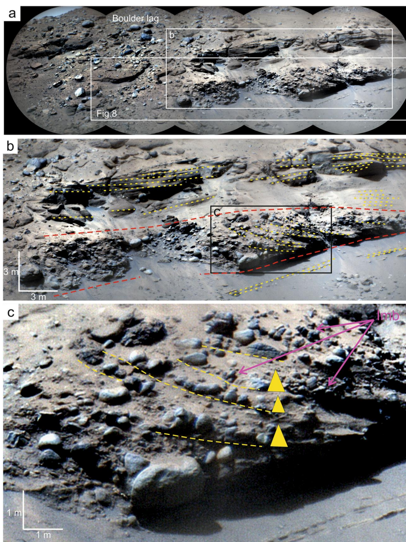
Figure 5. (a) SuperCam Remote Micro-Imager mosaic of five images on the Miners Castle outcrops. (b) Close-up of the central part of the outcrops with boulder conglomerates overlain by sandstones (with local cobbles). Yellow dotted line indicates bedding planes. Red dashed lines indicate approximate limits of the conglomerates. Note that the base of the conglomerates seems concordant to the layers of sandstones, without truncations. (c) Detailed view of the cobble and boulder-rich section of conglomerates displaying imbricated cobbles that bound individual beds (yellow dashed lines) with fining upward texture (yellow triangles). Imb indicates imbrication of clasts.
