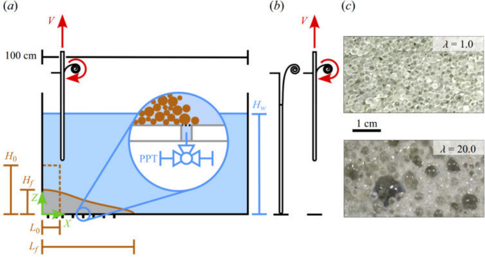
Figure 1. Sketch of the column collapse experimental set-up. (a) Side view highlighting the column initial and final heights and lengths ( H_0, L_0 ) and ( H_f, L_f ), respectively. Note that L_0 \approx 8.5 cm for all experiments, and for immersed collapses the water level is H_w \approx 50 cm. The inset shows the set-up for the basal pore pressure transducer (PPT) placed at X = [3, 7, 10, 15, 20, 25, 30, 35] cm and Y = 9 cm. (b) The release mechanism. The column collapses after removing a gate vertically with velocity V \approx 0.85 m s -1 . The gate is pulled by rapidly rolling a PTFE film, reducing shear on the face contacting the grains. (c) Close-up lateral views of the glass bead granular systems with size ratios \lambda = d_{max}/d_{min} = 1 and 20, where d_{min} and d_{max} are the minimum and maximum grain diameters, respectively.
