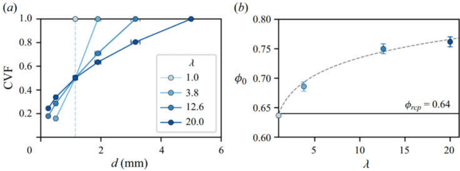
Figure 2. (a) The CDF as a function of the grain diameter d with a distribution following CVF = (d/d_{max})^n with n = [1, 1.38, 0.69, 0.47] for the size ratios \lambda = [1, 3.8, 12.6, 20] , respectively. All GSDs have common CDF 0.5 for d_{50} = 1.15 mm. Markers represent the mean size, and horizontal bars represent the ranges in size reported by the supplier. (b) Average sample initial packing fraction \phi_0 as a function of \lambda . The vertical error bars represent the variability among samples with the same polydispersity level. The dashed line follows a power-law function in the form \phi_0 = \lambda^{0.06} \phi_{rcp} , with \phi_{rcp} being the random close packing of monodisperse spheres (Scott 1960).
