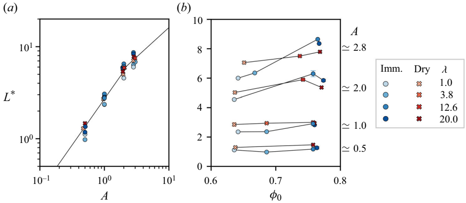
Figure 7. Normalized final runout L^* = (L_f - L_0)/L_0 as a function of (a) A and (b) \phi_0 . The lines in (a) indicate L^* = aA^b , with the values (a, b) = (2.7, 1.0) for short columns ( A < 2 ) and (a, b) = (3.7, 0.64) for tall columns ( A \geq 2 ). Error bars indicate variability between repetitions.
