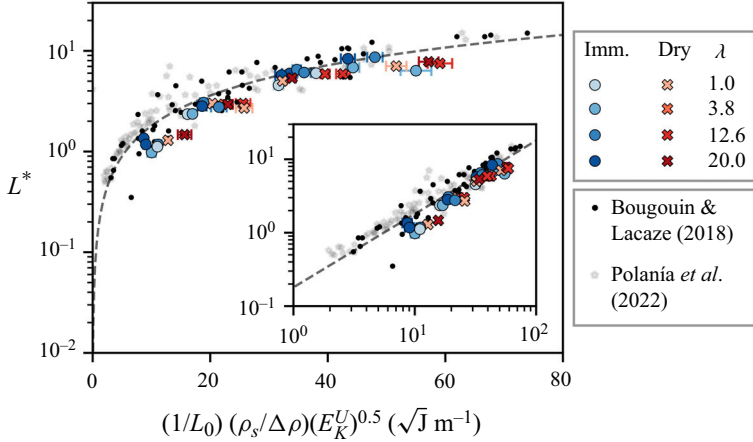
Figure 10. Scaling of the normalized final runout L^* with the column kinetics according to (4.1). Here, E_K^U = MU^2/2 is the column kinetic energy during the steady propagation, M = L_0 H_0 \phi_0 \rho_s is the column mass with unitary width, and \phi_0 is the initial column packing fraction. This scaling is compared with previous experimental and numerical results (Bougouin & Lacaze 2018; Polanía et al. 2022). The horizontal error bars show the variability associated with U . The dashed line follows a trend of power index 1.
