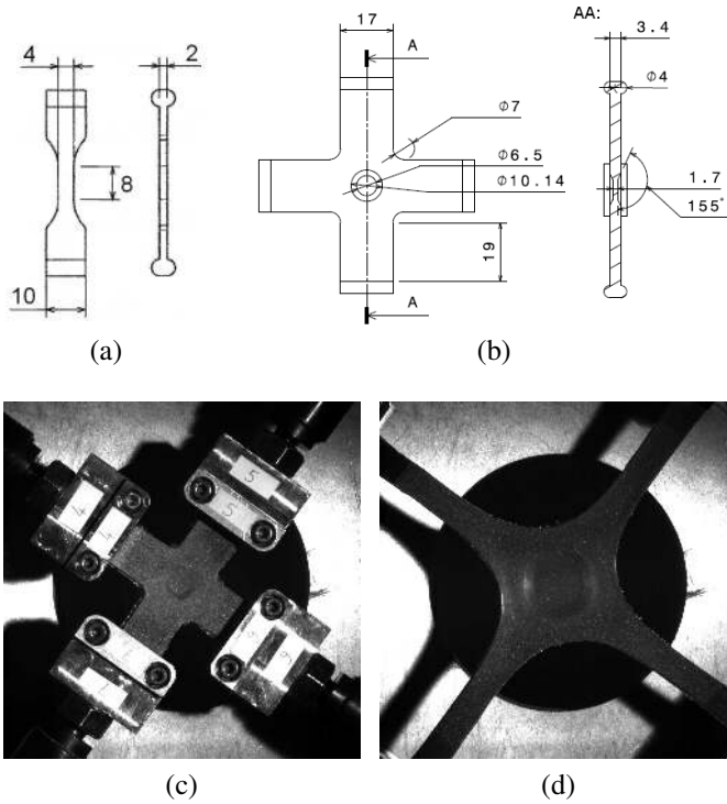
Figure 1: Dimensions of the (a) uniaxial samples and (b) biaxial samples. Cruciform sample (c) in undeformed state and (d) in equibiaxial deformation state.
