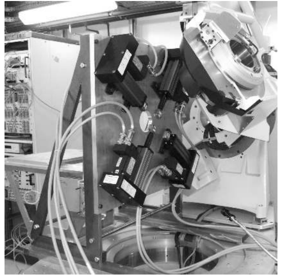
Figure 2: Uniaxial and biaxial stretching machine in DiffAbs.
