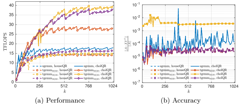
Fig. 3. Performance and accuracy of randLRA with refinement. (In (b), \text{tgemm}_{32|32} and \text{tgemm}_{16|32} completely overlap both for Householder QR and Cholesky QR).
