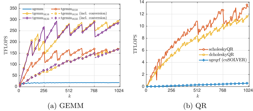
Fig. 1. Performance of the GEMM and QR kernels.
