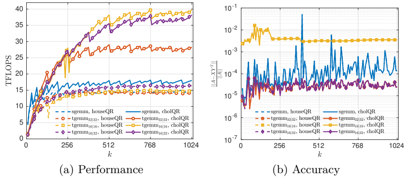
Fig. 3. Performance and accuracy of randLRA with refinement. (In (b), \text{tgemm}_{32|32} and \text{tgemm}_{16|32} completely overlap both for Householder QR and Cholesky QR).
