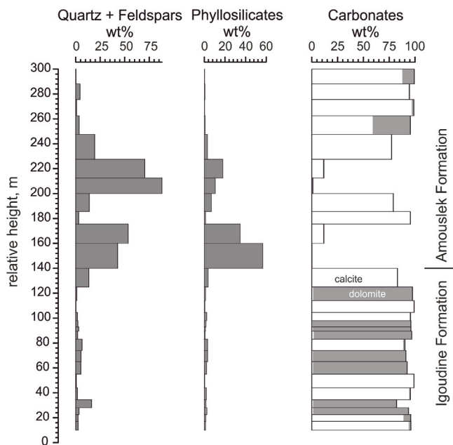
Fig. 3. Mineral composition of the studied samples. Quartz + feldspars (quartz, K-feldspar, plagioclase), phyllosilicates (K-mica, chlorite), carbonate (calcite, dolomite). Calcite content is shown with white bars and dolomite content with gray bars.
