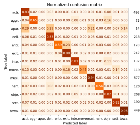
(b) distilcamembert-base, 10% of data
