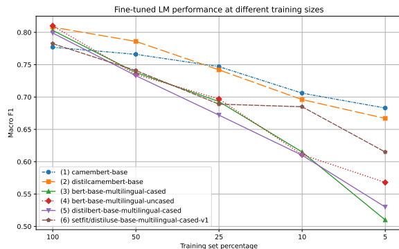
Figure 1: LM performance as training set is reduced
