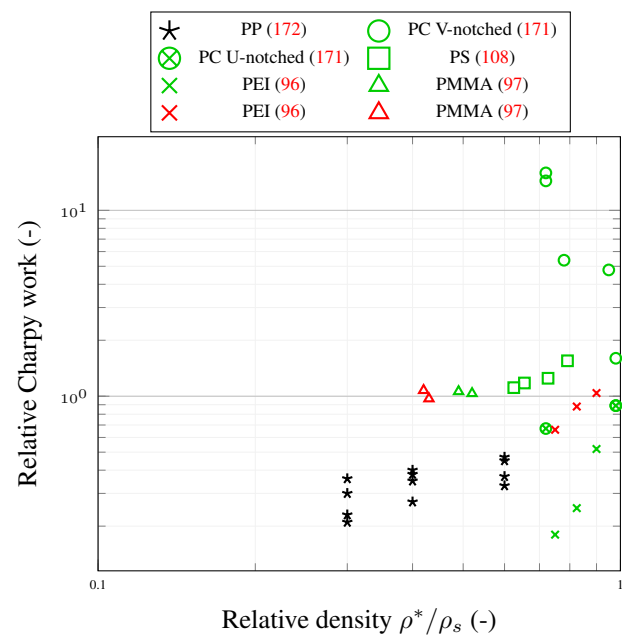
Figure 15. Relative data obtained from Charpy impact as a function of relative density. In black, mesocellular foams. In green, microcellular foams. In red, nanocellular foams (log-log scale).
