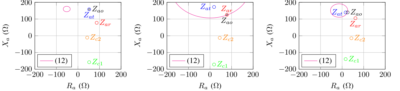
Fig. 4. Impedance matching maximizing the read range for (a) Impinj Monza 2 chip ( K = 0.013 ), (b) Impinj Monza X-8K chip ( K = 0.39 ) and (c) Impinj Monza R6-P chip ( K = 0.083 ).
