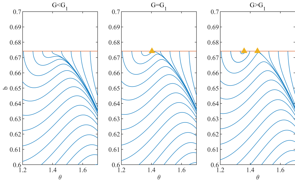
Figure 2: Phase plot for \mu = 0.1 , \epsilon = 0.01 , \zeta = 0.01 , \kappa = 1 , \lambda = 0.1 and \sigma = 1 for three values of G around G_1 = 0.0101 . Solid red line corresponds to b = b_1 and orange triangle to the folded singularities.
