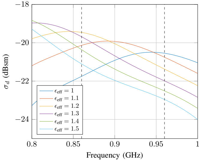
Fig. 7. Delta RCS as a function of the frequency for different effective dielectric permittivity values.
