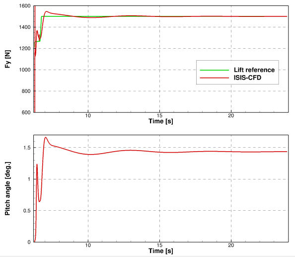
Fig. 4. F_y^* = 1500 \text{ N} , \text{Re} = 4.70 \times 10^6 , U_\infty = 56.7 \text{ ms}^{-1} : Evolution of lift force (top) and pitch angle (bottom) versus the time
