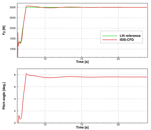
Fig. 5. F_y^* = 3000 \text{ N} , \text{Re} = 4.70 \times 10^6 , U_\infty = 56.7 \text{ ms}^{-1} : Evolution of lift force (top) and pitch angle (bottom) versus the time
