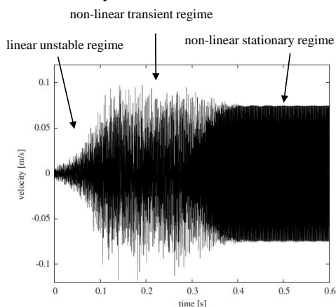
Figure 2: Typical time history of self-sustained vibrations [4].
