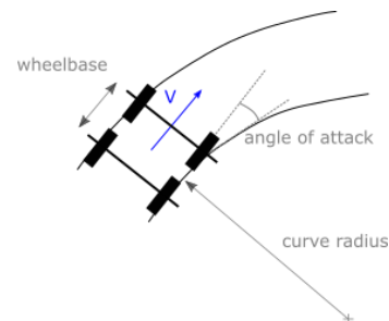
Figure 1: Railway curve negotiation.
