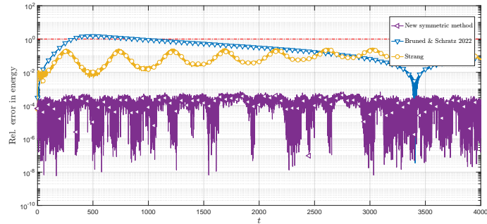
(b) Low regularity data, u_0 \in H^2 and M = 64 .
