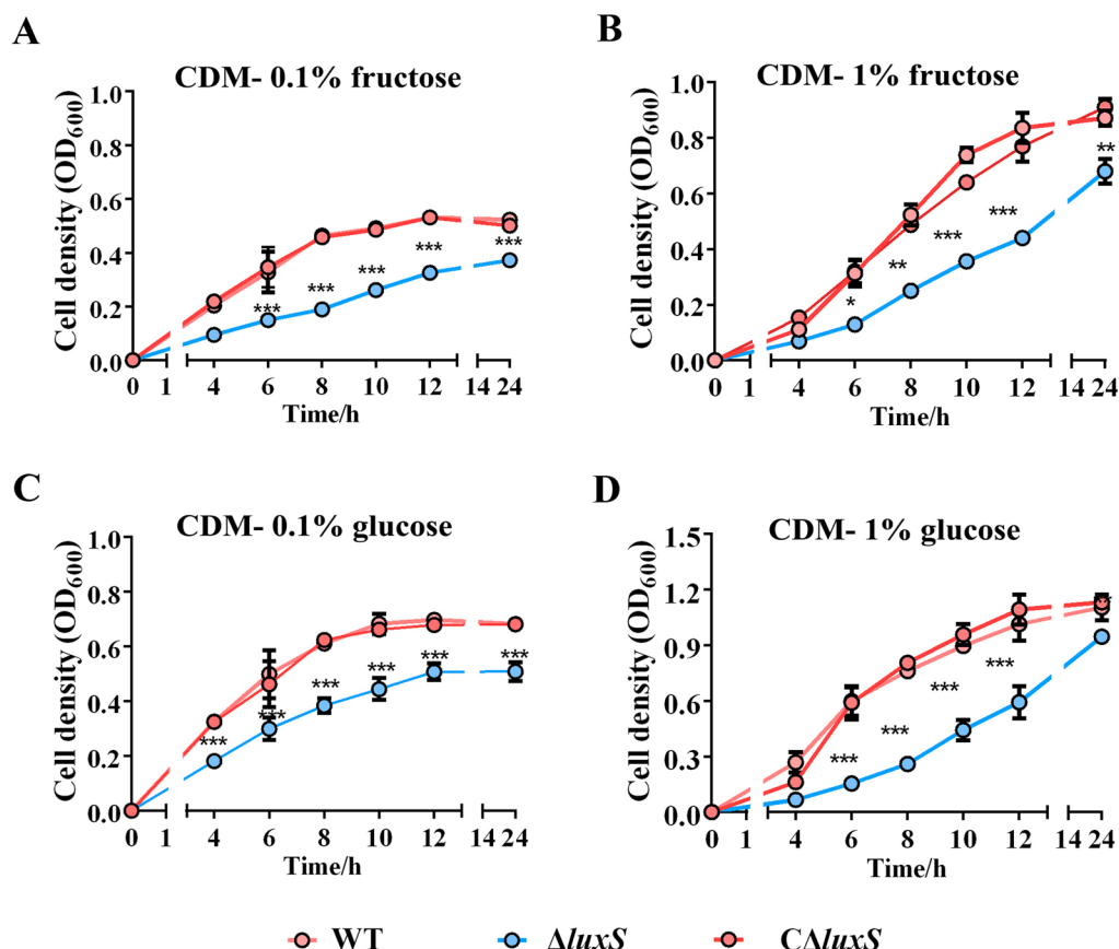
Fig. 2 Influence of luxS deficiency on carbon source availability of S. agalactiae strains. All strains were cultivated in a chemically-defined medium (CDM) supplemented fructose (A, B) or glucose (C, D) at a range of concentrations from 0.1% to 1% (w/v) as the sole carbon source, separately. Data are presented as the mean \pm SD for three independent experiments. * P < 0.05 , ** P < 0.01 , or *** P < 0.001 , indicates a significant difference between the indicated strain and the WT strain.
