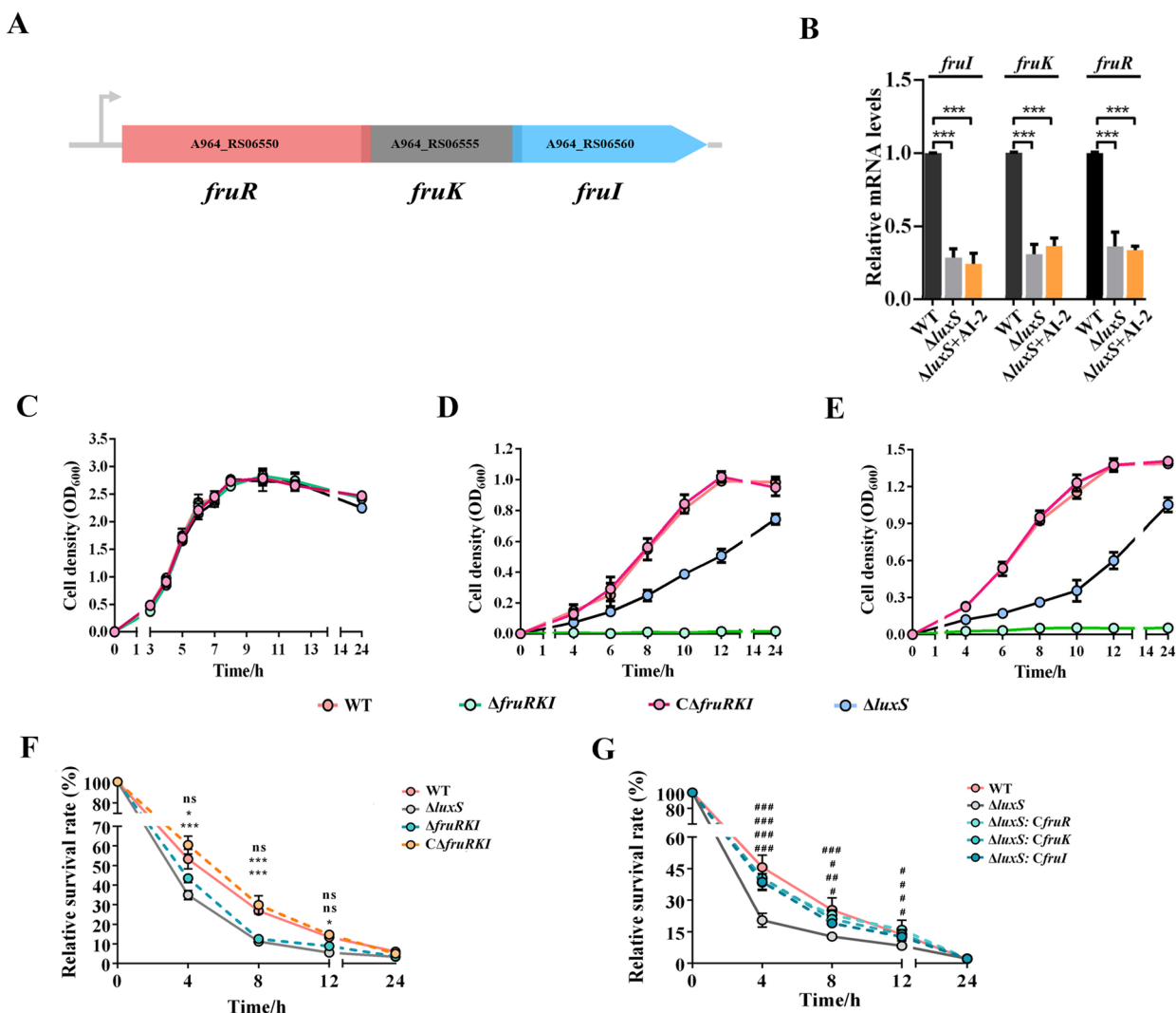
Fig. 3 Growth characters and intramacrophage survival capabilities of S. agalactiae strains. A Genetic structure of the fruRKI operon in S. agalactiae . B Relative mRNA levels of the fruRKI genes. C Growth curves of the WT, \Delta luxS , \Delta fruRKI and C\Delta fruRKI strains cultivated in THB. D Growth curves of the WT, \Delta luxS , \Delta fruRKI and C\Delta fruRKI strains cultivated in CDM supplemented 1% fructose. E Growth curves of the WT, \Delta luxS , \Delta fruRKI and C\Delta fruRKI strains cultivated in CDM supplemented 1% glucose. F Intracellular survival of the WT, \Delta luxS , \Delta fruRKI and C\Delta fruRKI strains in macrophages. G Intracellular survival of the WT, \Delta luxS , \Delta luxS:: fruI , \Delta luxS:: fruK and \Delta luxS:: fruR strains in macrophages. Data are presented as the mean \pm SD of three independent experiments. * P < 0.05 or *** P < 0.001 , indicates a significant difference between the indicated strain and the WT strain. # < 0.05 , ## < 0.01 , or ### < 0.001 , indicates a significant difference between the indicated strain and the \Delta luxS strain.
