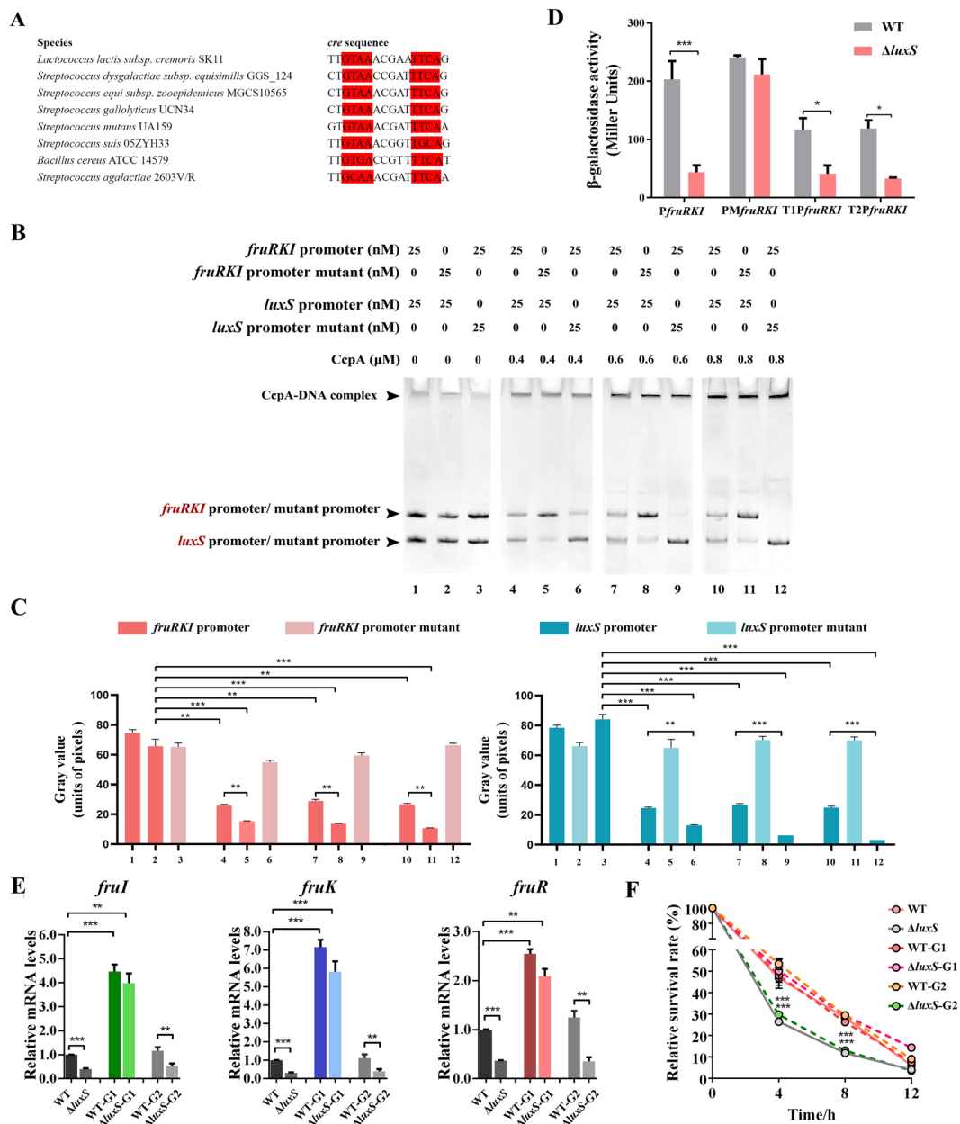
Fig. 6 luxS indirectly regulates the expression of fruRKI operon through the cre region in the fruRKI promoter. A The sequence alignment of cre from eight gram-positive bacteria. The conserved regions of cre are highlighted. B Competitive binding of the luxS promoter and the fruRKI promoter to CcpA by EMSA analysis. The 129-bp fragment of luxS promoter was tested for its ability to bind with CcpA (0.4, 0.6 and 0.8 μM) in presence of 188-bp fragment of wild type fruRKI promoter (lane 4, 7 and 10) or fruRKI promoter with mutations on cre (lane 6, 9 and 12); the 188-bp fragment of fruRKI promoter was tested for its ability to bind with CcpA (0.4, 0.6 and 0.8 μM) in presence of 129-bp fragments of wild type luxS promoter (lane 4, 7 and 10) or luxS promoter with mutations on cre (lane 5, 8 and 11); Lane 1 to 3. Different components of internal controls. C The DNA-binding capacity of CcpA was measured with grayscale analysis of the blots. D The fruRKI promoter activity in the WT and \Delta luxS strains containing the P \Delta fruRKI -lacZ reporter plasmid. The WT and \Delta luxS strains containing T1P \Delta fruRKI -lacZ or T2P \Delta fruRKI -lacZ reporter plasmids serve as control groups. The \beta -galactosidase activity was expressed as relative miller units. E Relative mRNA levels of the fruRKI genes determined by real-time PCR. WT-G1: eight-base substitution in the cre conserve region of fruRKI promoter in WT; \Delta luxS -G1: eight-base substitution in the cre conserve region of fruRKI promoter in \Delta luxS ; WT-G2: eight-base substitution in the cre non-conserve region of fruRKI promoter in WT; \Delta luxS -G2: eight-base substitution in the cre non-conserve region of fruRKI promoter in \Delta luxS . F Intracellular survival rates of the WT, \Delta luxS , WT-G1, \Delta luxS -G1, WT-G2 and \Delta luxS -G2 strains in macrophages. Data are presented as the mean \pm SD of three independent experiments. * P < 0.05 , ** P < 0.01 , or *** P < 0.001 .
