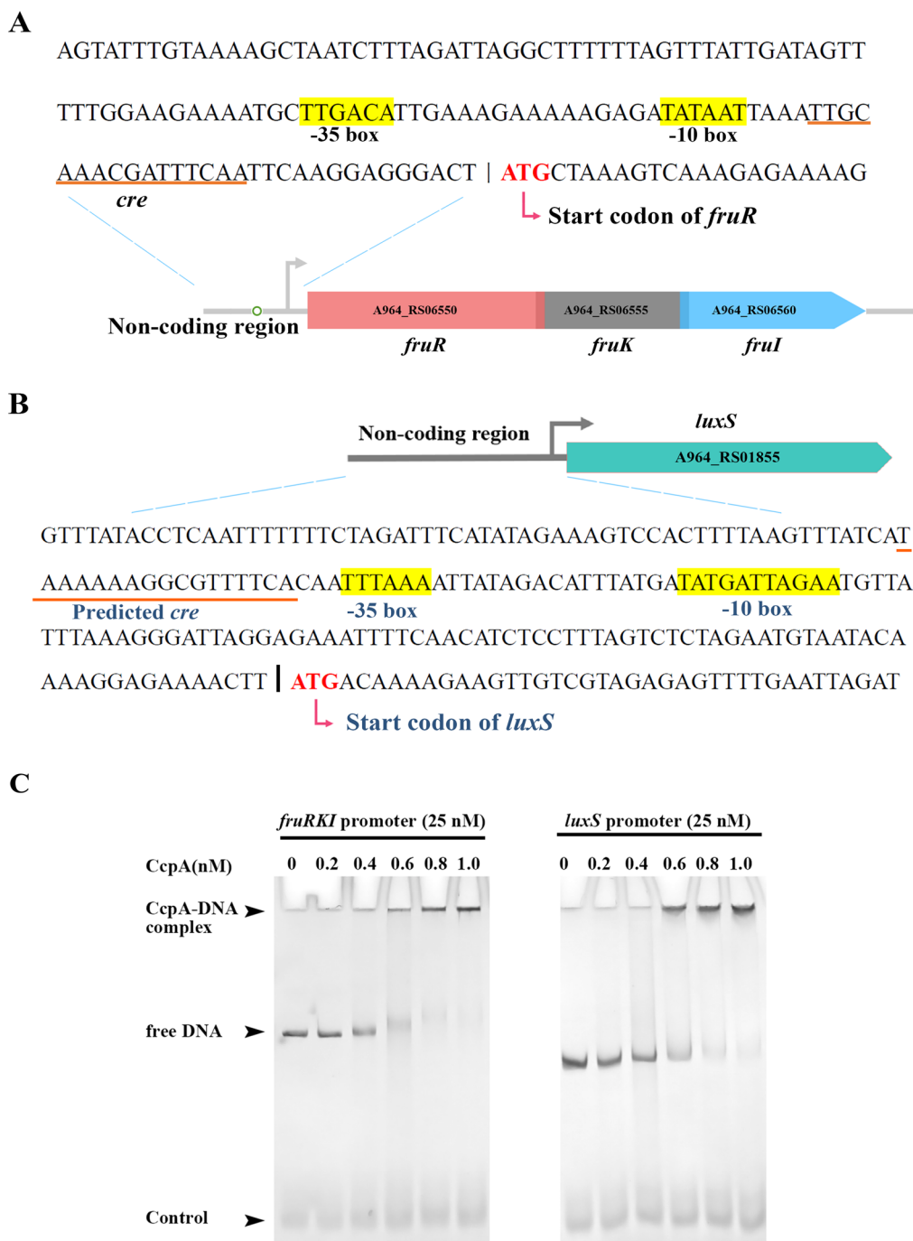
Fig. 5 The in vitro binding of CcpA to the fruRKI promoter or luxS promoter. A Diagrams depicting the noncoding region of the fruRKI operon. The magnified region indicates the promoter sequences, including the putative cre for CcpA binding (underlined), and the -10 and -35 positions are highlighted and labeled. B Diagrams depicting the noncoding region of the luxS gene. The putative cre is underlined, and the -10 and -35 positions are highlighted and labeled. C An electrophoretic mobility shift assay (EMSA) showing the binding ability of CcpA protein to the fruRKI or luxS promoters (25 nM). The concentrations of CcpA ranged from 0 to 1.0 μM.
