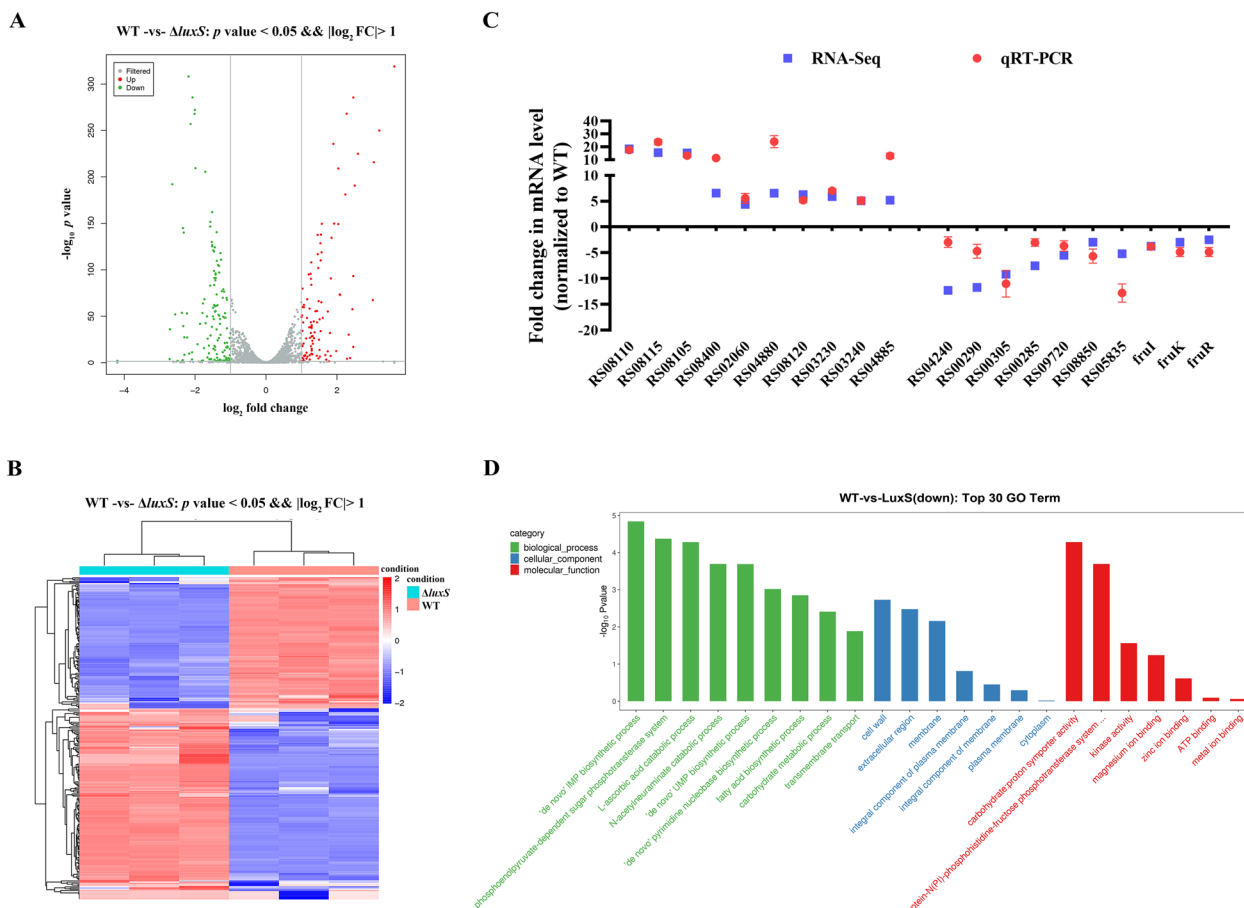
Fig. 1 Comparative transcriptomics analysis. A Volcano plot of the differentially expressed genes. The x-axis represents fold change ( \log_2 ) and y-axis represents p -value ( \log_{10} ). Red dots represent upregulated genes and green dots indicate downregulated genes with a significant difference. B Heat map of gene expression. A total of 264 genes were differentially expressed in the \Delta luxS strain compared to the wild-type (WT) strain. Red and blue fonts represent up- and down-regulated genes, respectively in the WT or \Delta luxS strains. C Relative mRNA levels of 20 differently expressed genes determined by RT-qPCR. Data are expressed as n-fold change normalized to mRNA level of WT. D Gene Ontology (GO) classification of downregulated genes in the \Delta luxS strain.
