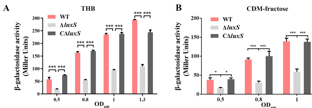
Fig. 4 The promoter activity of fruR KI in S. agalactiae strains grown in rich medium or chemically defined medium (CDM). A The fruR KI promoter activity in the WT, \Delta luxS and C\Delta luxS strains cultivated in THB (rich medium). B The fruR KI promoter activity in the WT, \Delta luxS and C\Delta luxS strains cultivated in CDM supplemented 1% fructose. Data are presented as the mean \pm SD of three independent experiments. *** P < 0.001 .
