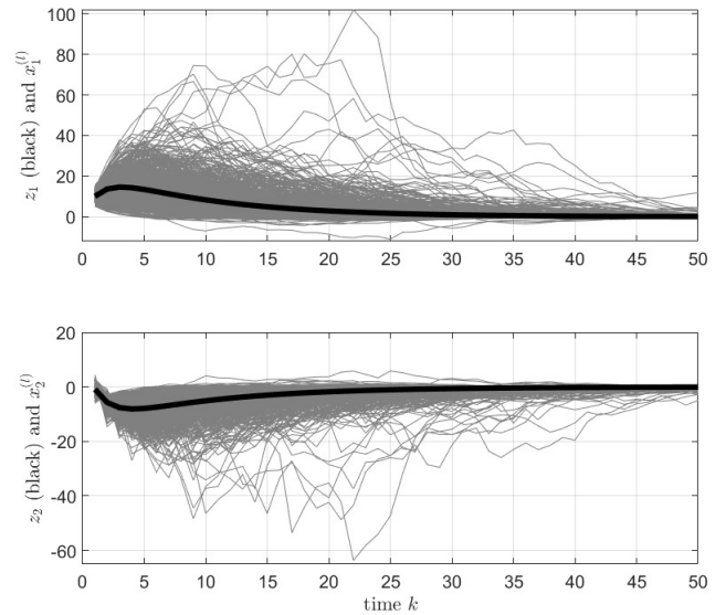
Fig. 2. The nominal and stochastic states z and x corresponding to system (18) using C_p as in (19), (up) The first components z_1 (in black) and x_1^{(l)} (in grey) for N = 1000 trials with l = 1, \dots, N , (bottom) The second components z_2 (in black) and x_2^{(l)} (in grey).
