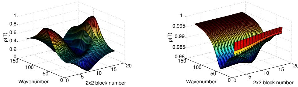
FIG. 6.1. Left: Spectral radius of T_j with \omega = \omega_{\text{op}} . Right: \omega = \omega_{\text{gen}} for C = 0.8 and \nu = 1 .
