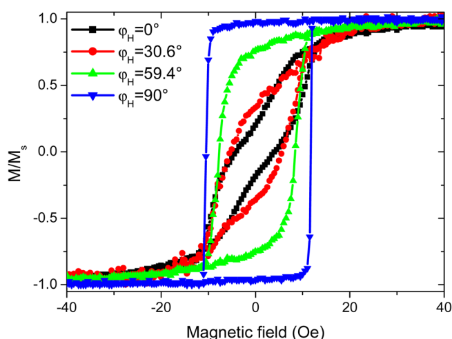
FIG. 2. (Color online) MOKE magnetization loops of the 10-nm-thick \text{Fe}_{1.7}\text{Ge} film. The magnetic field is applied parallel to the film surface, at various angles ( \varphi_H ) with the [11\bar{2}0]_{\text{FeGe}} axis.
