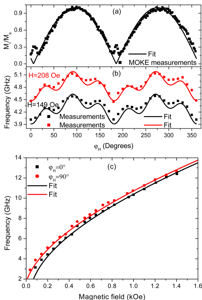
FIG. 3. (Color online) The 10 nm-thick \text{Fe}_{1.7}\text{Ge} film: (a) MOKE reduced remanent magnetization ( M_r/M_s ), (b) in-plane angular dependence of the resonance frequency and (c) in-plane field dependence of the frequency of uniform precession mode. All the fits (full lines) are obtained using the parameters indicated in the Table I.
