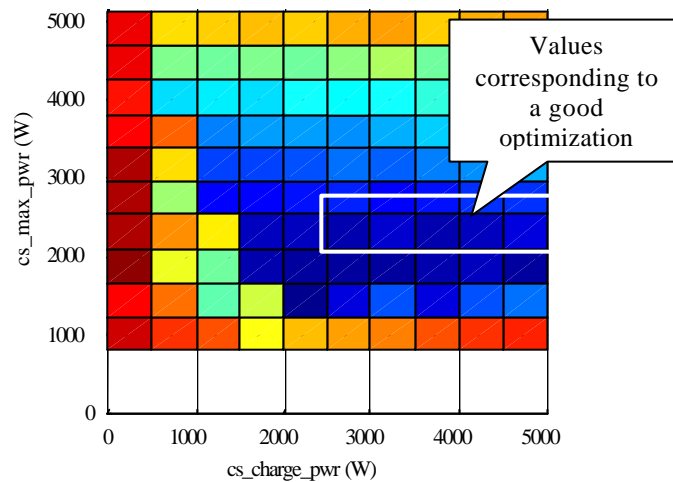
Fig. 7: Computation of the parameters cs_max_pwr and cs_charge_pwr for the urban driving schedule
