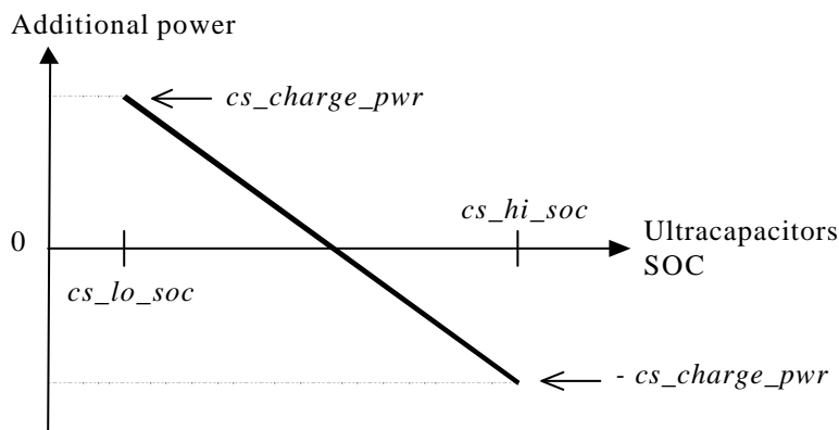
Fig. 6 : Computation of additional power for ultracapacitors SOC correction
