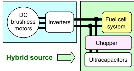
Fig. 2 : Structure of the vehicle drive train
