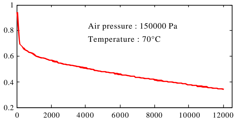
Fig. 3 : Graph showing the voltage [V] of a cell as a function of current density [A/m 2 ] (polarization curve)
