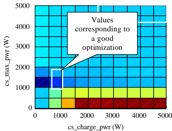
Fig. 8 : Computation of the parameters cs_max_pwr and cs_charge_pwr for the constant speed driving schedule
