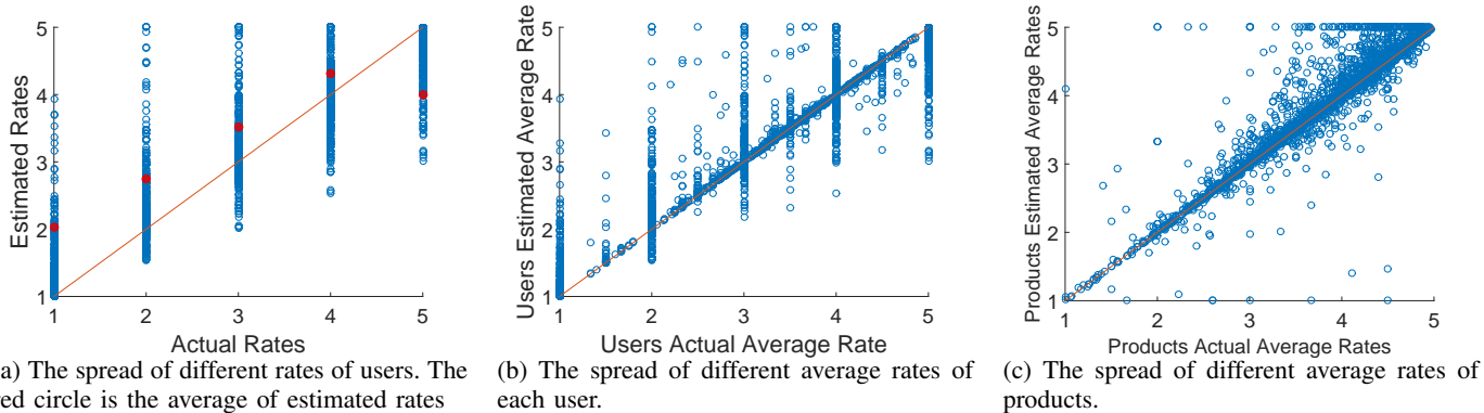
Fig. 3: Epinions dataset
