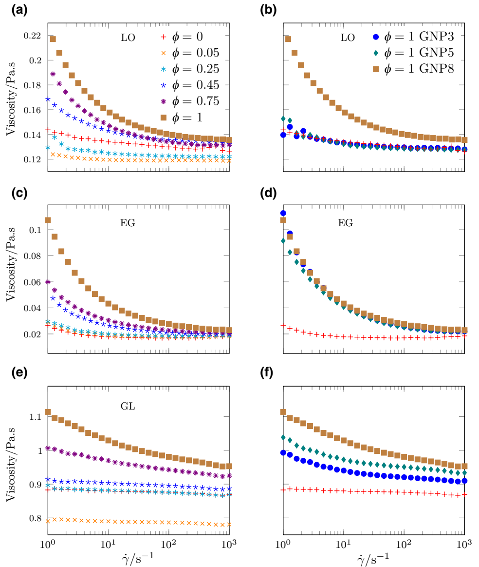
Fig. 12 Viscosity of LO+GNP, EG+GNP and GL+GNP solutions as a function of shear rate \dot{\gamma} , a, c, e for different \phi of GNP8 and b, d, f for different SSA at \phi = 1\% and 25\text{ }^\circ\text{C} (298.15 K)
