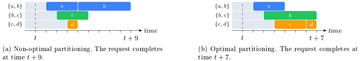
Fig. 2: Two possible partitions of a multi-get request released at time t . The gray areas represent the current load of each machine, while the sets written on the left represent the values stored on each machine. In the first case, the opsets are \{a, b\} , \{c\} and \{d\} , which causes imbalance. In the second case, the opsets are \{a\} , \{b\} and \{c, d\} , which is the best possible choice for the current multi-get request.
