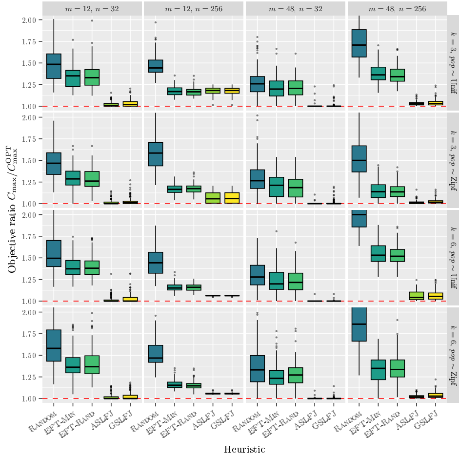
Fig. 10: Ratio between the makespan C_{\max} given by each heuristic and the optimal makespan C_{\max}^{\text{OPT}} in different settings (the lower the better). Each boxplot aggregates 100 iterations. The red line represents the baseline.
