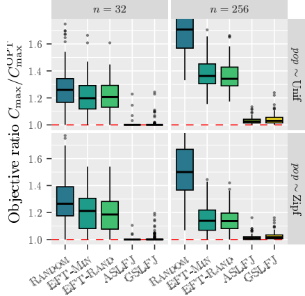
(a) Ratio between C_{\max} and C_{\max}^{\text{OPT}} .
