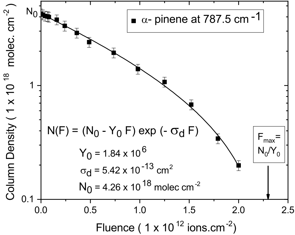
Figure 6. Column density evolution of \alpha -pinene as a function of fluence for the band 787.5 \text{ cm}^{-1} .
