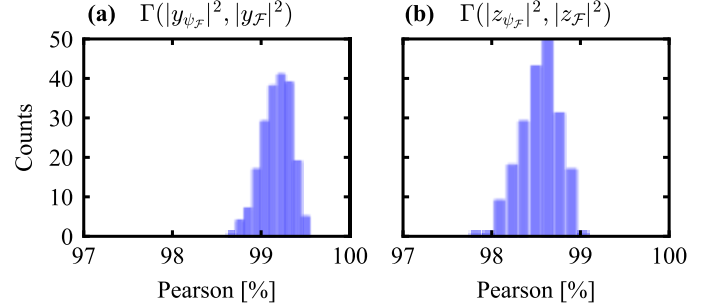
Fig. 8. Distribution of Pearson correlation coefficients between predicted and experimental intensities from the testing dataset in near field (a) and far field (b).
