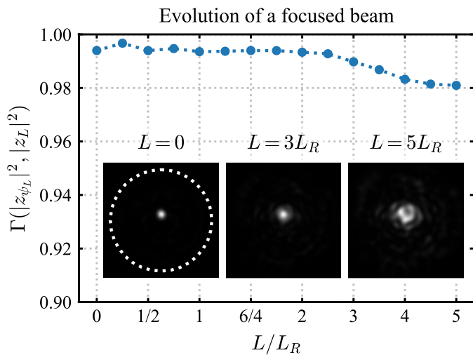
Fig. 9. Experimental data – Example of focused beam at the fiber output, optimized from the experimental MT. Evolution of the Pearson correlation between the experimental images |z_L|^2 and the predicted ones |z_{\psi_L}|^2 along the propagation axis. L_R : Rayleigh length of the focused beam. Dashed white circle defines the fiber core.
