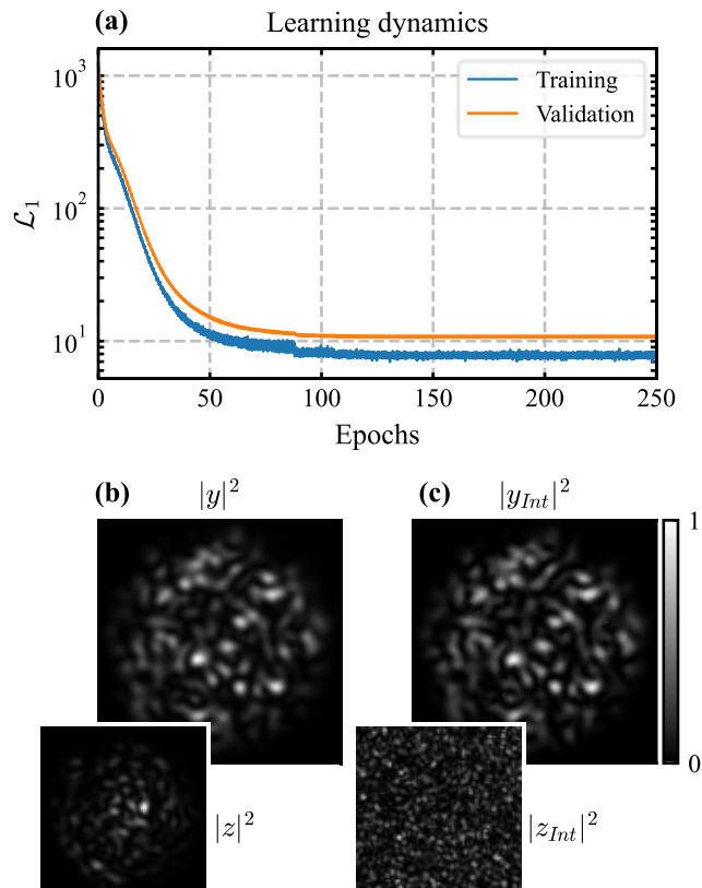
Fig. 6. Experimental data – (a) Learning dynamics as a function of epochs. Convergence is reached in about 150 epochs with 32-mini batch size and a learning rate starting at 0.05. It lasts about 200s with our Pytorch implementation using a laptop computer with a NVIDIA RTX A1000 4GB GPU and an Intel i7-12700H 2.30 GHz CPU. (b)-(c) Experimental and predicted near field intensities. Insets show the corresponding experimental and predicted far field intensities.
