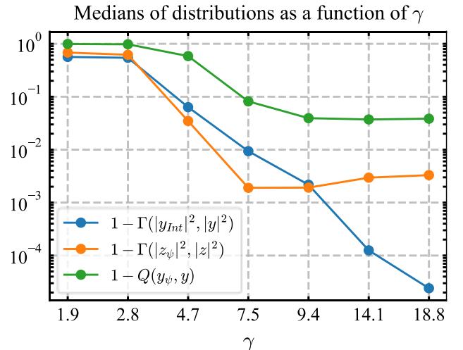
Fig. 4. Median of the metric distributions as a function of the ratio \gamma = N^t/n . Blue: Pearson correlation coefficient between the predicted and ground truth near field intensities. Orange: Pearson correlation coefficient between the predicted and
