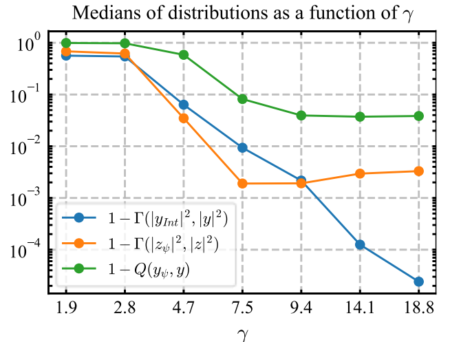
Fig. 4. Median of the metric distributions as a function of the ratio \gamma = N^t/n . Blue: Pearson correlation coefficient between the predicted and ground truth near field intensities. Orange: Pearson correlation coefficient between the predicted and
