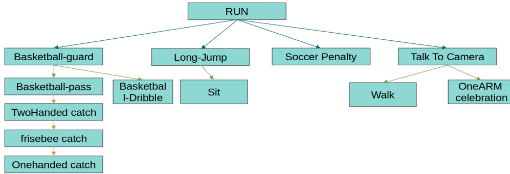
Figure 1. An example of human non-sequential dependencies. For instance, the actions RUN and OneHanded Catch are highly correlated but distant. Also the same start action RUN can lead to many different actions and scenarios. Therefore, it is very hard for online action detection or action anticipation to detect such relations without access to the future. In JOADAA, we propose to tackle this limitation by introducing a pseudo-future information by combining action anticipation and online action detection in the same task.
