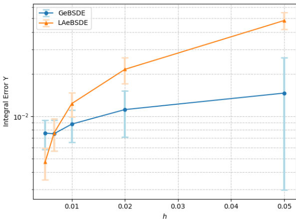
FIGURE 4. Integral error on Y over [0, T_H] .
