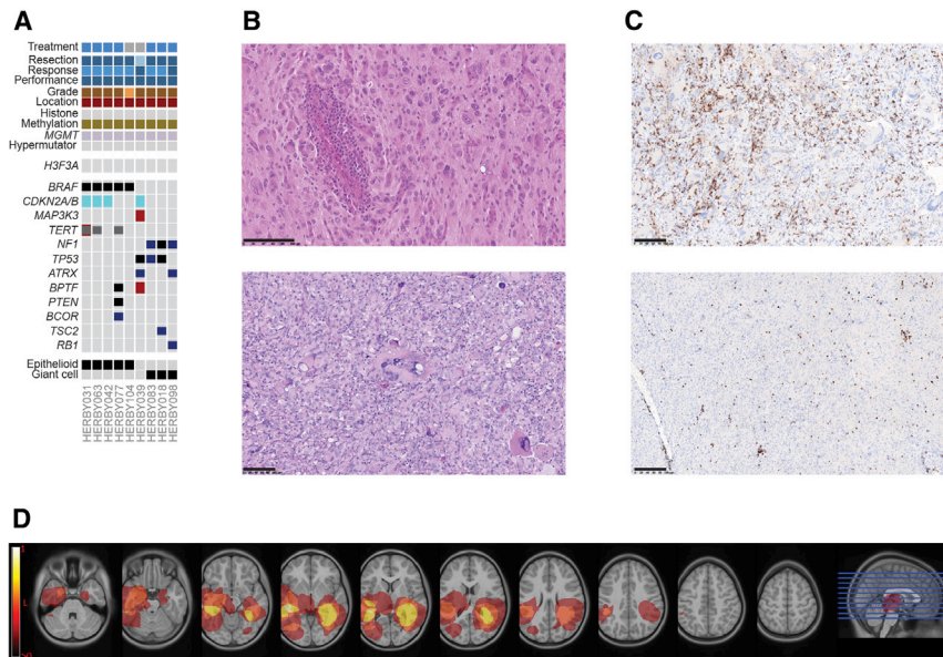
Figure 6. PXA-like Tumors
