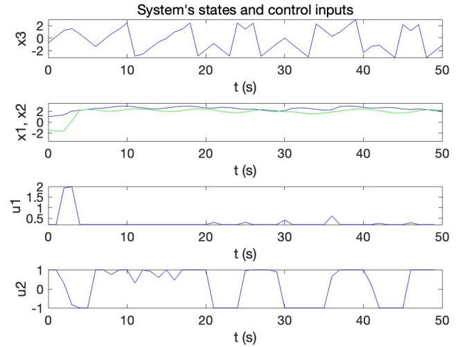
Fig. 4: Evolution of system's states and control inputs for (d) in Figure 5
