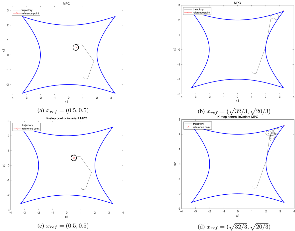
Fig. 5: Trajectory of moving carts. The upper two figures show the NMPC approach without terminal constraints and the two figures below show the NMPC using a K -step control invariant set ( K=5 ) as terminal constraint.
