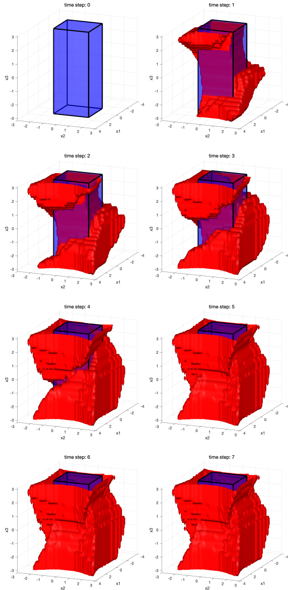
Fig. 3: The evolution of the set CPref_{[1:K]} (red parts) with K is depicted in the figure, where K = 0, 1, 2, \dots, 7 . By the fifth iteration step, the hyperrectangle is completely contained in the computed states, and by the seventh iteration step, the computed states are identical to the maximum control invariant set.
