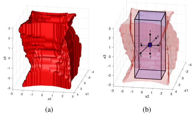
Fig. 2: On the left is the approximation of the maximal control invariant set computed using symbolic control, on the right is the stretching method, the direction of stretching is in order 1-6.
