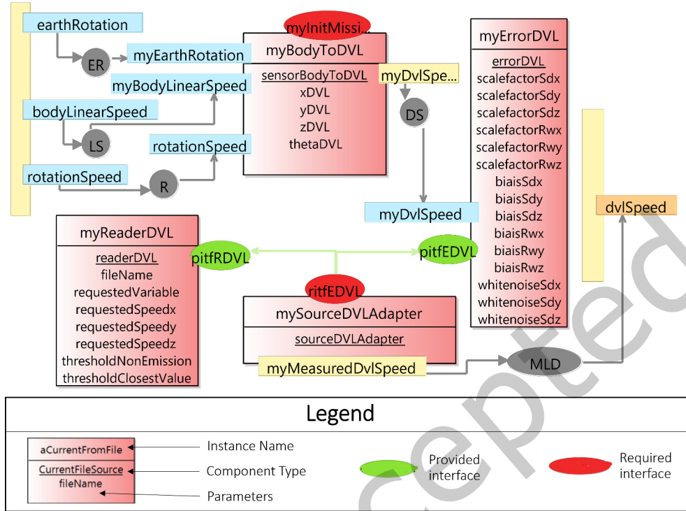
Fig. 6. DVL composite component.
