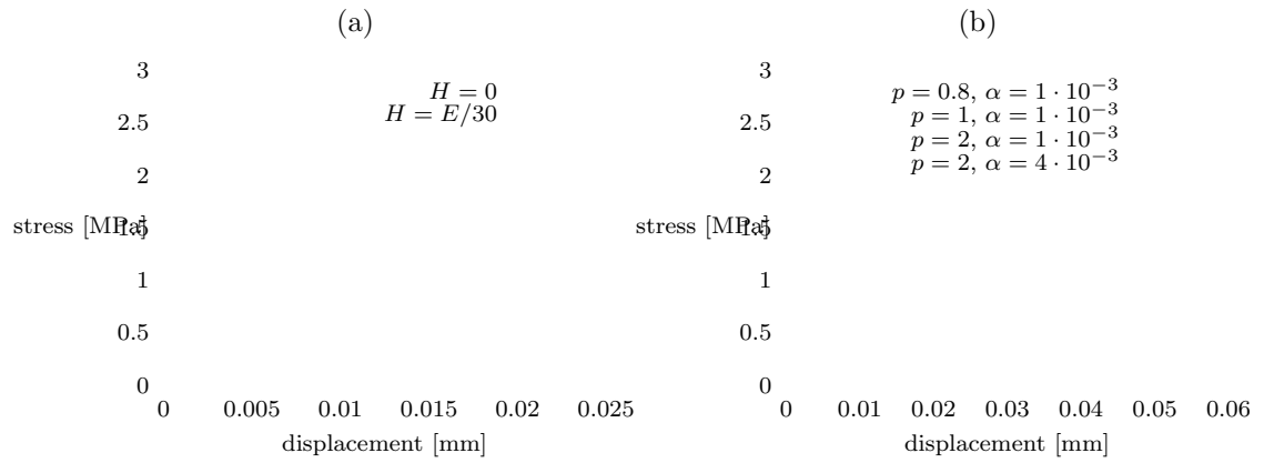
Figure 6: Stress-displacement diagrams for DMIS: (a) version 1, (b) version 2
