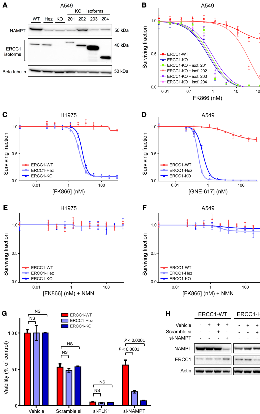
Figure 4. Exquisite sensitivity to NAMPT inhibition is a primary effect of ERCC1 deficiency. (A) Representative Western blot of NAMPT and ERCC1 protein expression and (B) survival experiment on FK866 exposure according to the reintroduction of the 4 alternative ERCC1 isoforms. (C) Survival experiment on FK866 exposure of the H1975 ERCC1-isogenic model. (D) Survival experiment on GNE-617 exposure of the A549 ERCC1-isogenic model. (E and F) Rescue of FK866 toxicity by the administration of nicotinamide mononucleotide (NMN) 100 μM in the H1975 (E) and A549 (F) ERCC1-isogenic models. Data for B–F are mean surviving fraction ± SD from 1 experiment. (G) Cell viability after acute NAMPT silencing by siRNA in A549 ERCC1-proficient and ERCC1-deficient cells. Toxicity of PLK1 silencing by siRNA was used as a positive control for cell death induction. Data are mean viability ± SD from 1 representative experiment. Statistical analyses are indicated (Mann-Whitney U test corrected for multiple comparisons). NS indicates no statistically significant difference. (H) Representative Western blot of NAMPT and ERCC1 protein expression after NAMPT silencing by siRNA in A549 ERCC1-proficient and ERCC1-deficient cells. For A–H, data were replicated in at least 3 independent experiments.
