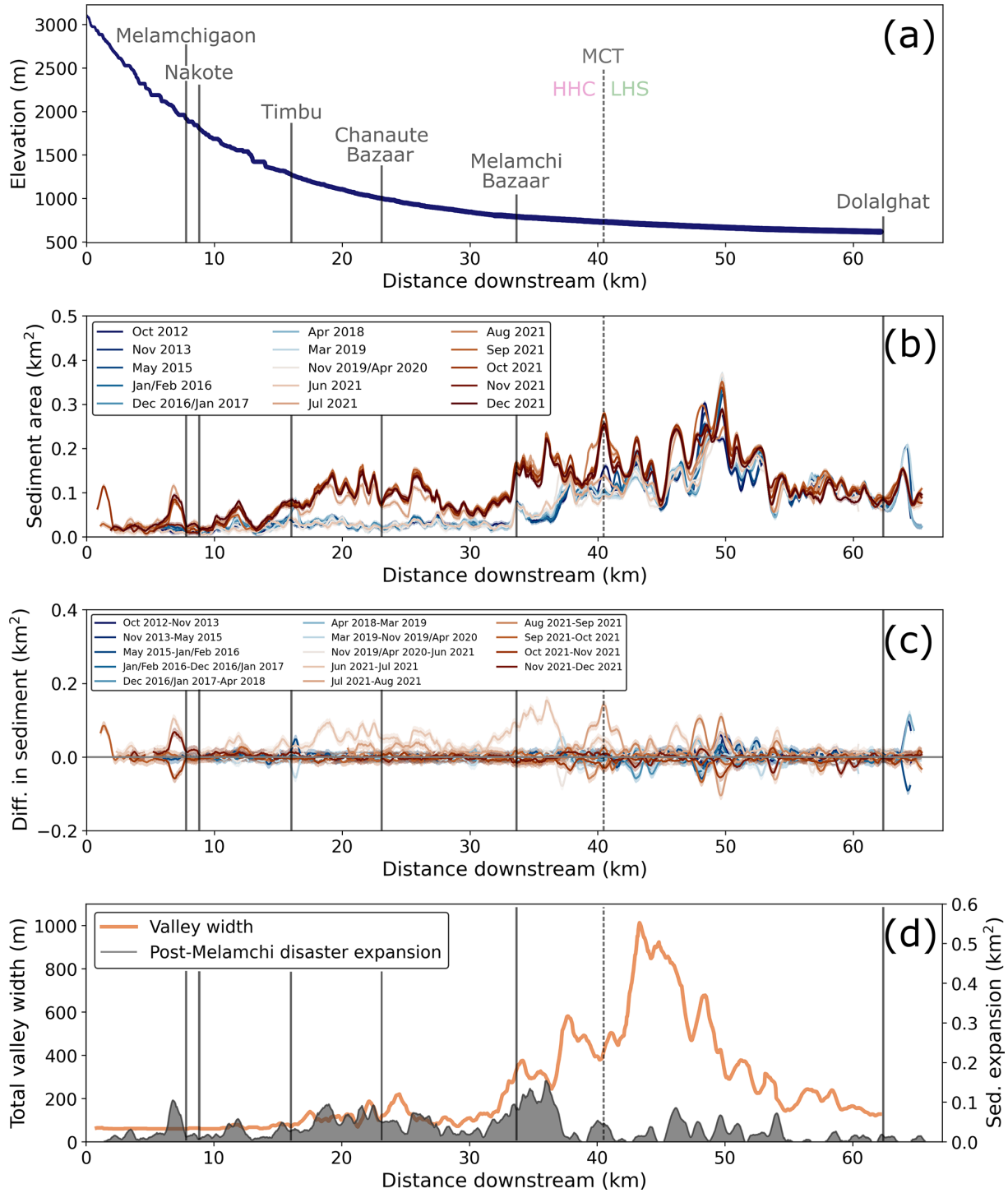
Figure 6. Changes in sediment area along the Melamchi–Indrawati rivers: (a) long profile of the Melamchi–Indrawati rivers within the study area, (b) mapped sediment area per 0.5 km 2 window along profile, (c) difference in mapped area along profile between each time period, and (d) valley width extracted with LSDTopoTools plotted alongside mapped expansion in sediment between June and July 2021 (i.e. difference in mapped sediment area before and after the Melamchi event). Areas until November 2019 or April 2020 inclusive are mapped in Google Earth Pro; areas from June 2021 onward are mapped in QGIS from Planetscope imagery. Locations mentioned in the text are labelled in (a) and shown with vertical grey lines. The dashed grey line indicates the approximate location of the Main Central Thrust (MCT), separating the Higher Himalayan Crystallines (HHC) from the Lesser Himalayan Sequence (LHS).
