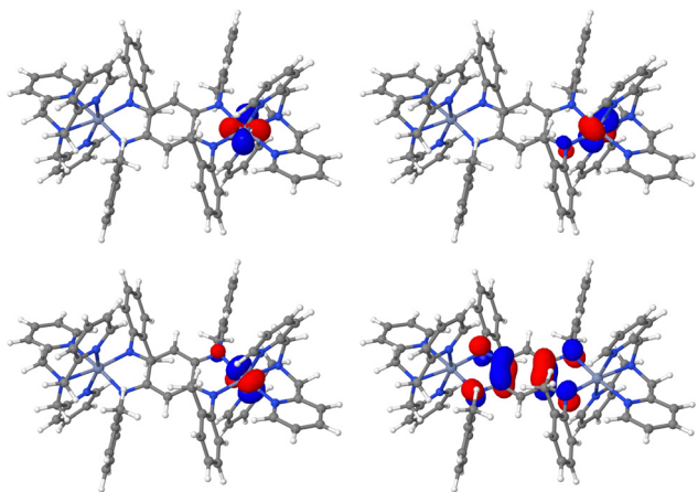
Fig. 2 Isosurface of the d_{xy} (top left), d_{yz} (top right), d_{xz} (bottom left) and \pi^* radical (bottom right) magnetic orbitals of 1a . Blue grey = chromium, blue = nitrogen, grey = carbon, white = hydrogen. Isovalue = 0.5 a.u.
