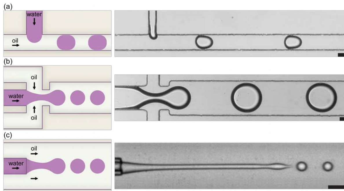
Figure 1 Examples of three common passive droplet generation modes.
