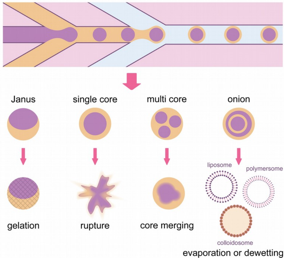
Figure 3 Multiple emulsion templating.
