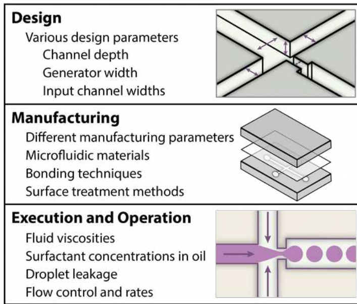
Figure 7 Summary of sources of variability in droplet-based microfluidic experimentation.
