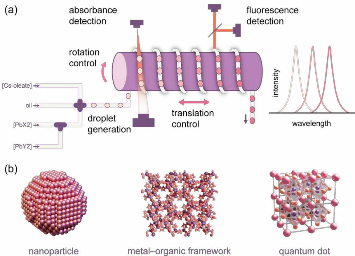
Figure 6 Droplet-based microfluidic synthesis of materials with bespoke properties.
