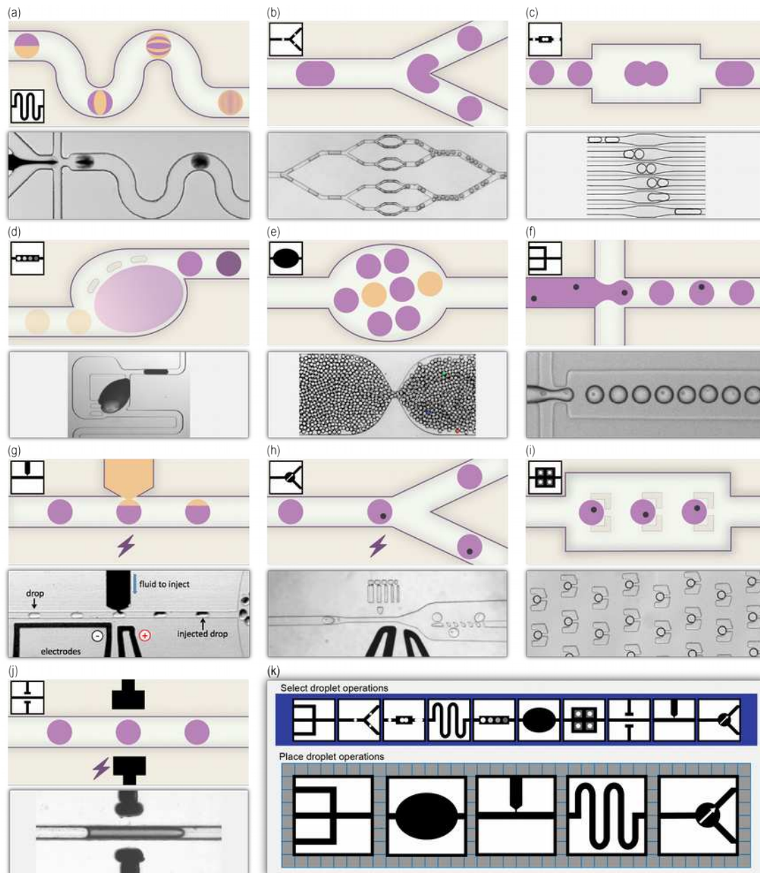
Figure 2 Droplet manipulations and unit operations.
