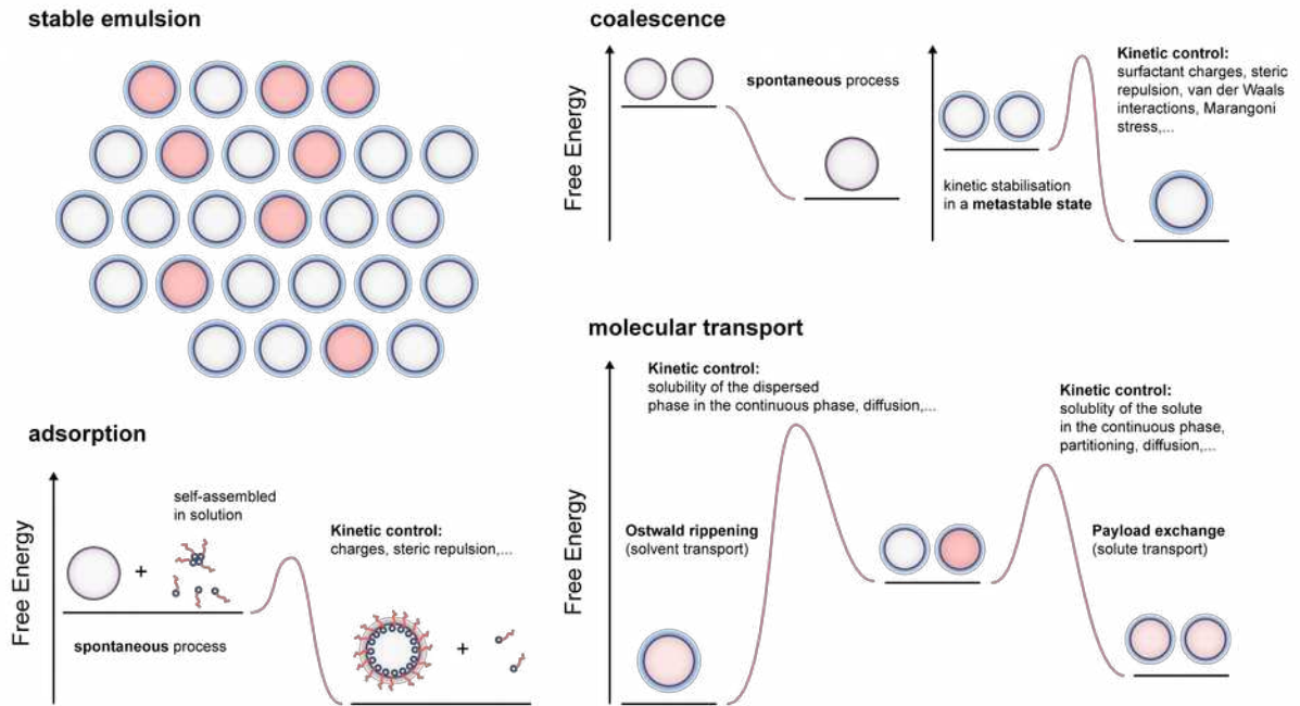
Figure 8 Physical phenomena affecting the stability of microfluidic emulsions.
