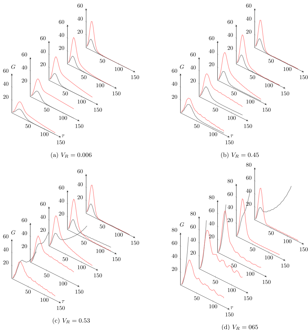
FIG. 5. G as a function of the target time \tau for Re = 6666 and (a) V_R = 0.006 , (b) V_R = 0.45 , (c) V_R = 0.53 , and (d) V_R = 0.65 . For all panels, the streamwise wavenumbers are \alpha = 0.8, 1, 1.2, 1.4, and 1.6 (from the left to the right). Red, sinuous symmetry; black, varicose symmetry.
