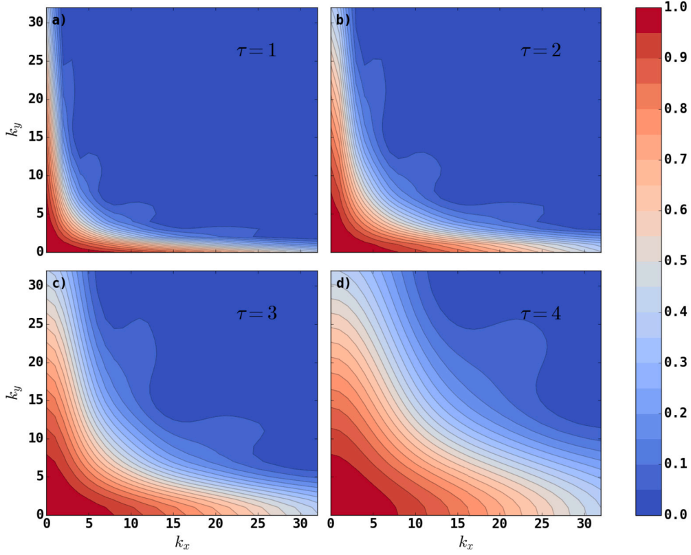
Fig. 11. Filters for order q = 1 and grid level p = 6 , for \tau = 1 (a), \tau = 2 (b), \tau = 3 (c) and \tau = 4 (d).
