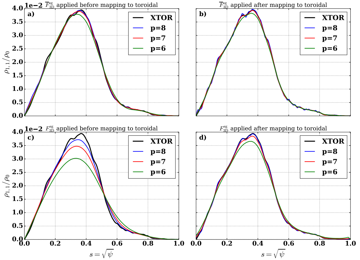
Fig. 7. Radial structure of the m = 1, n = 1 mode. Filtering before the mapping and with \bar{F}_{3D}^{sg} (a), after the mapping and with \bar{F}_{3D}^{sg} (b), before the mapping and with F_{3D}^{sg} (c), after the mapping and with F_{3D}^{sg} (d).
