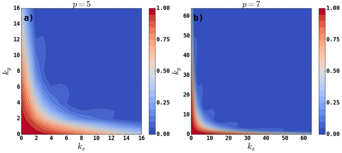
Fig. 4. Comparison between the sparse grid filters for p = 5 (a) and p = 7 (b).
