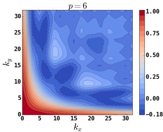
Fig. 13. Sparse grid filter for a grid level p = 6 when the shape function is the hat function (order 0).
