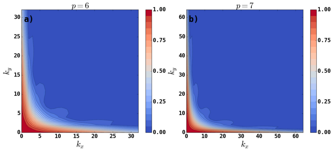
Fig. 1. Sparse grid filter in two dimensions for p = 6 (a) and p = 7 (b). (For interpretation of the colors in the figure(s), the reader is referred to the web version of this article.)
