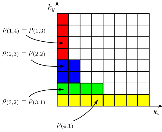
Fig. 5. Selection of retained modes (nodes in contact with colored squares) in the Fourier sparse grid algorithm ( p = 4 ).
