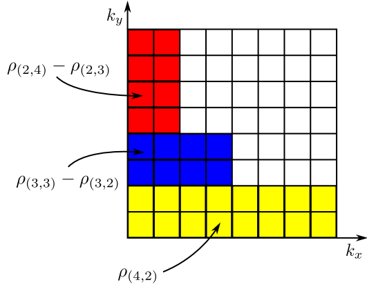
Fig. 12. Selection of retained modes (nodes in contact with colored squares) in the Fourier sparse grid algorithm ( p = 4 , \tau = 2 ).
