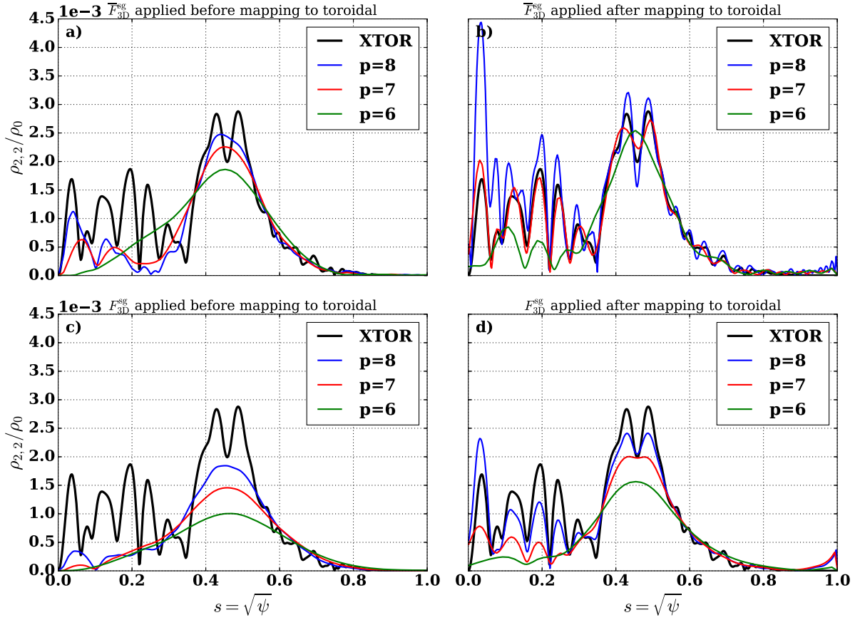
Fig. 10. Radial structure of the m = 2, n = 2 mode. Filtering before the mapping and with \overline{F}_{3D}^{\text{sg}} (a), after the mapping and with \overline{F}_{3D}^{\text{sg}} (b), before the mapping and with F_{3D}^{\text{sg}} (c), after the mapping and with F_{3D}^{\text{sg}} (d).
