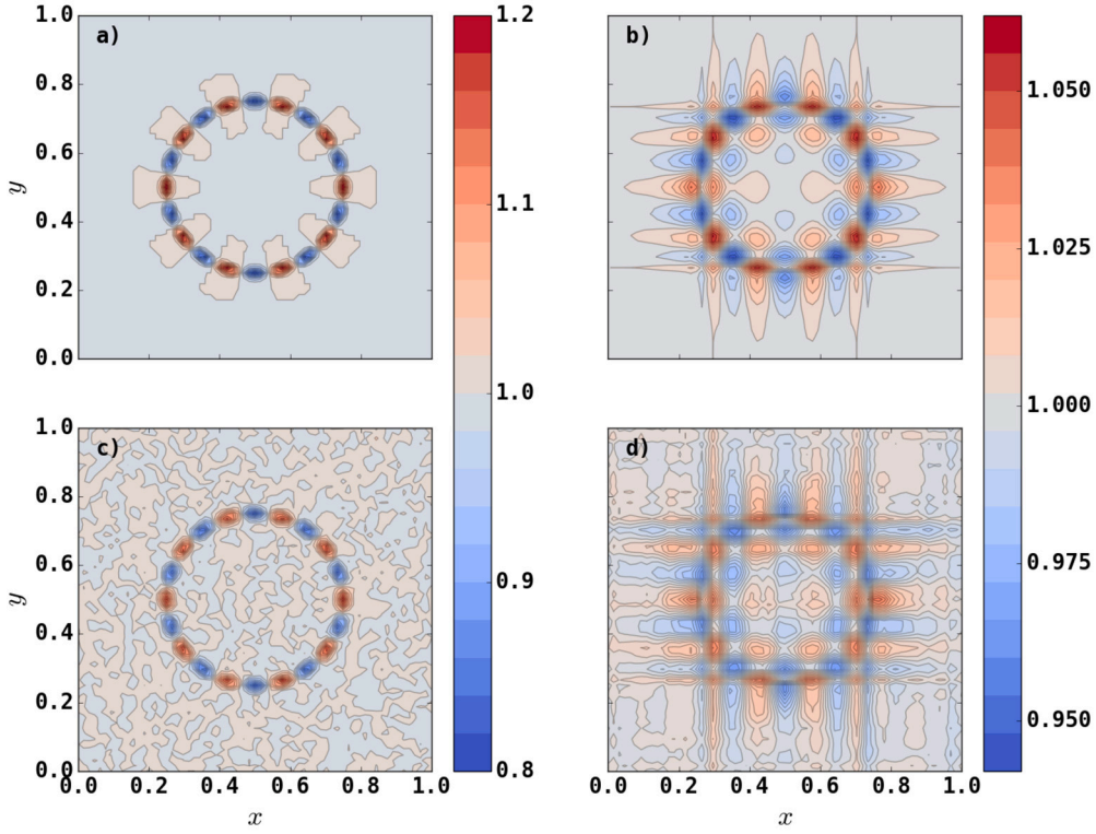
Fig. 2. Sparse grid deformation of an island structure. Analytical signal (a), sparse grid filtered analytical signal (b), density moment collected with N_p = 4 \times 10^7 markers using standard PIC method on a grid of level p = 6 (c), and using the sparse grid combination technique with the same level for the finest grid (d).
