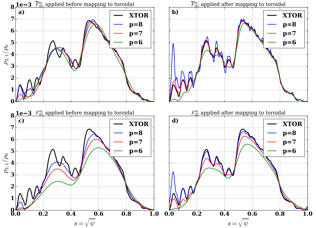
Fig. 9. Radial structure of the m=2, n=1 mode. Filtering before the mapping and with \overline{F}_{3D}^{sg} (a), after the mapping and with \overline{F}_{3D}^{sg} (b), before the mapping and with F_{3D}^{sg} (c), after the mapping and with F_{3D}^{sg} (d).
