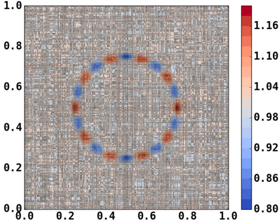
Fig. 3. Sparse grid PIC sampling of the island structure with N_p = 4 \times 10^7 markers, on a grid of level p = 10 ( 1024 \times 1024 ).
