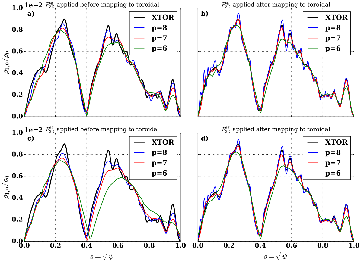
Fig. 8. Radial structure of the m = 1, n = 0 mode. Filtering before the mapping and with \bar{F}_{3D}^{sg} (a), after the mapping and with \bar{F}_{3D}^{sg} (b), before the mapping and with F_{3D}^{sg} (c), after the mapping and with F_{3D}^{sg} (d).
