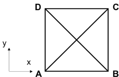
Fig. 5. Base unit cell with the beams AB, BC, CD, AD, AC and BD.
