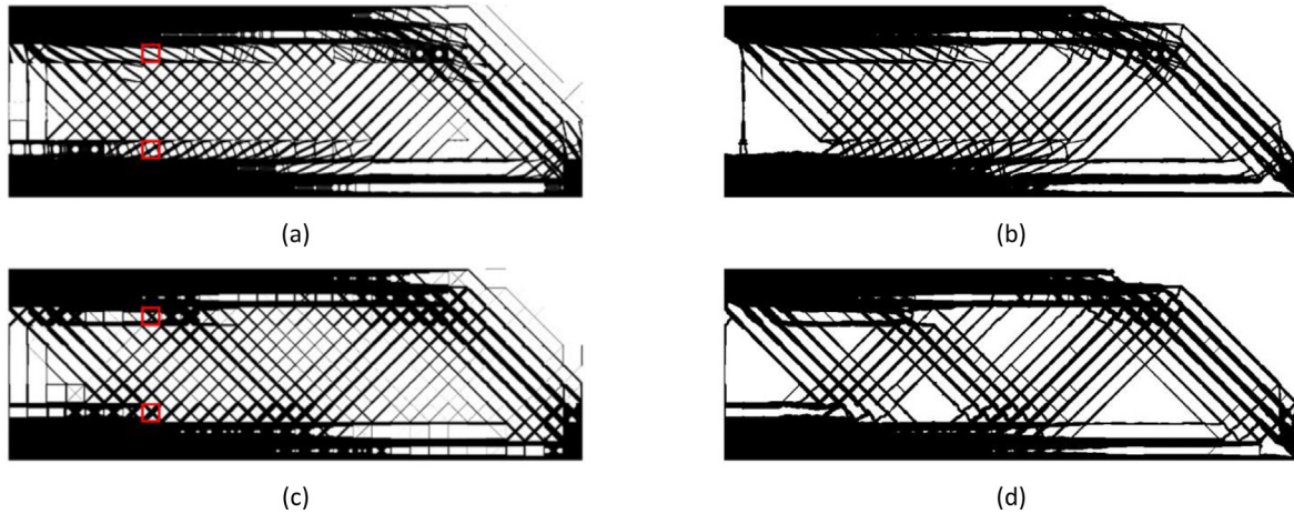
Fig. 15. Comparison of MBB designs with 100 \times 100 cells for the compliance minimization: (a) and (b) original EMTO respectively without post-processing and with post-processing, (c) and (d) Ex-EMTO respectively without post-processing and with post-processing.
