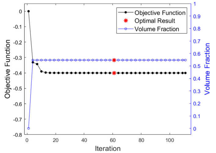
Fig. 10. Iteration history for the example in Figure 9.
