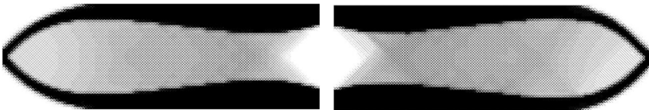
(a) Design obtained by varying only the density with the new database. The theoretical compliance is equal to 186.
