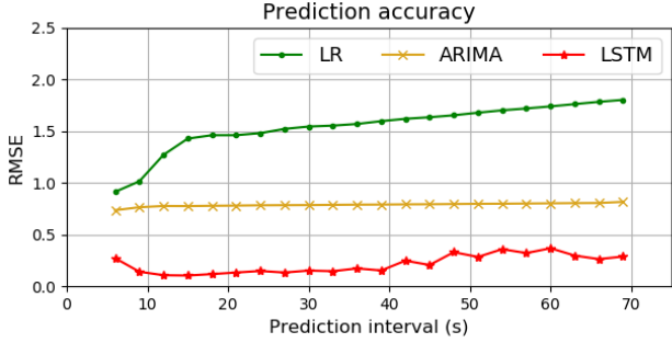
Figure 12: RMSE of LSTM, ARIMA and LR prediction methods
