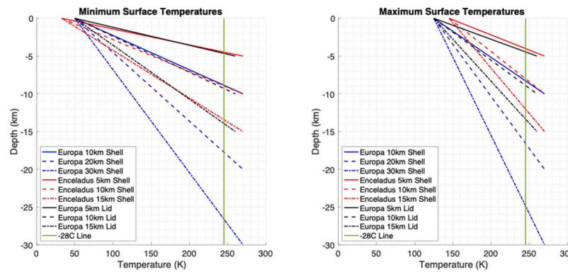
Fig. 5. Model results of ice shell thermal profiles and their intersection with the -28^{\circ}\text{C} limit of life (green line) for a) minimum and b) maximum surface ice temperatures. Variations in ice shell/brittle lid thickness are represented by line types (solid, dashed, dot-dashed) for both Europa (blue/black) and Enceladus (red).
