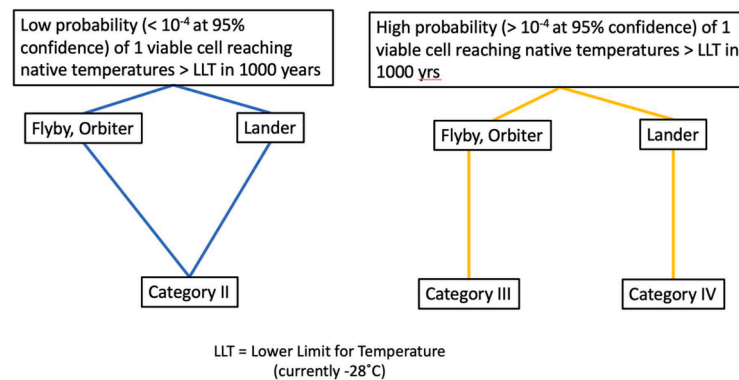
Fig. 4. Decision tree for categorization of orbiters and landers with regards to the lower limit for replication of Earth life.
