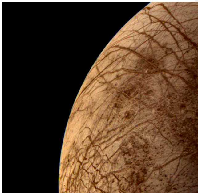
Fig. 2. Color image of Europa acquired by Voyager 2 during its closest approach on July 9, 1979. Image credit NASA/JPL https://www.jpl.nasa.gov/images/pia00459-europa-during-voyager-2-closest-approach .
