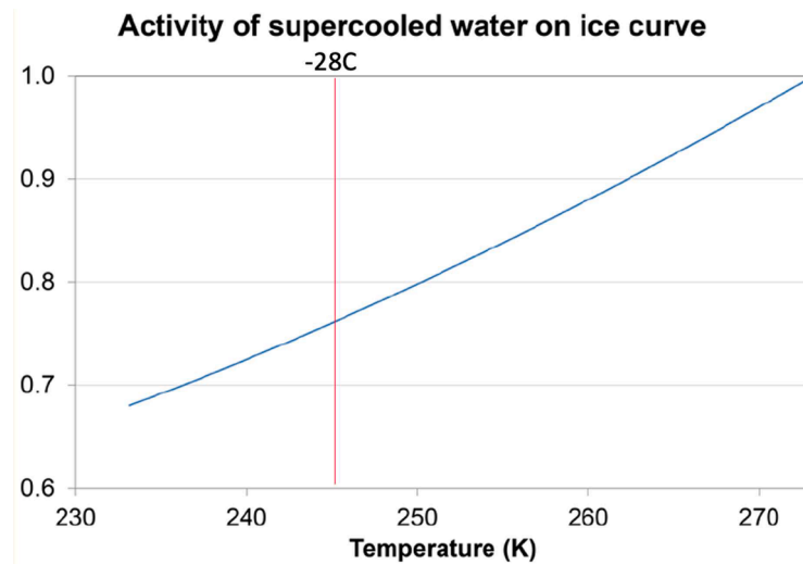
Fig. 3. Modeled temperature vs water activity in pure ice (blue line). Red vertical line shows the water activity at the current established lower temperature limit for Earth life in COSPAR policy. Modified from Sippola & Taskinen (2018).
