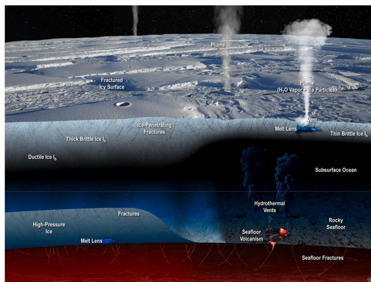
Fig. 1. Plumes and overturn of a fractured ice shell are means of exchanging matter between surface and ocean and volcanism, vents, and infiltration of fractured crust are means of exchange between ocean and core within icy satellites. From National Academies of Sciences, Engineering, and Medicine (2023). Courtesy P. Byrne.
