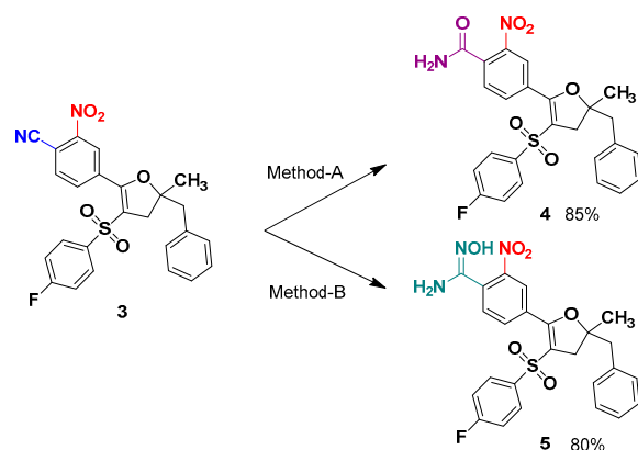
Scheme 3. Influence of the reaction conditions on the amide and the amidoxime synthesis. Method-A: 4 equiv. \text{NH}_2\text{OH}\cdot\text{HCl} , 2 equiv. \text{Na}_2\text{CO}_3 , EtOH, \text{N}_2 , 90 °C, MW, 1 h. Method-B: 10 equiv. \text{NH}_2\text{OH}\cdot\text{HCl} , 10 equiv. \text{KO}t\text{Bu} , DMSO, \text{N}_2 , 0 °C to RT, 18 h.
