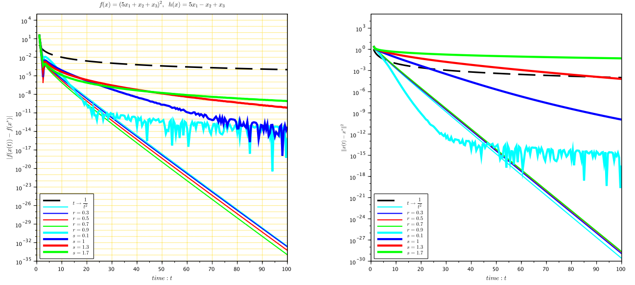
FIGURE 3. Here we compare the convergence rates for different values of 0 < r < 1 in system (MIPDALS), and those of 0 < s < 2 in system (51).
