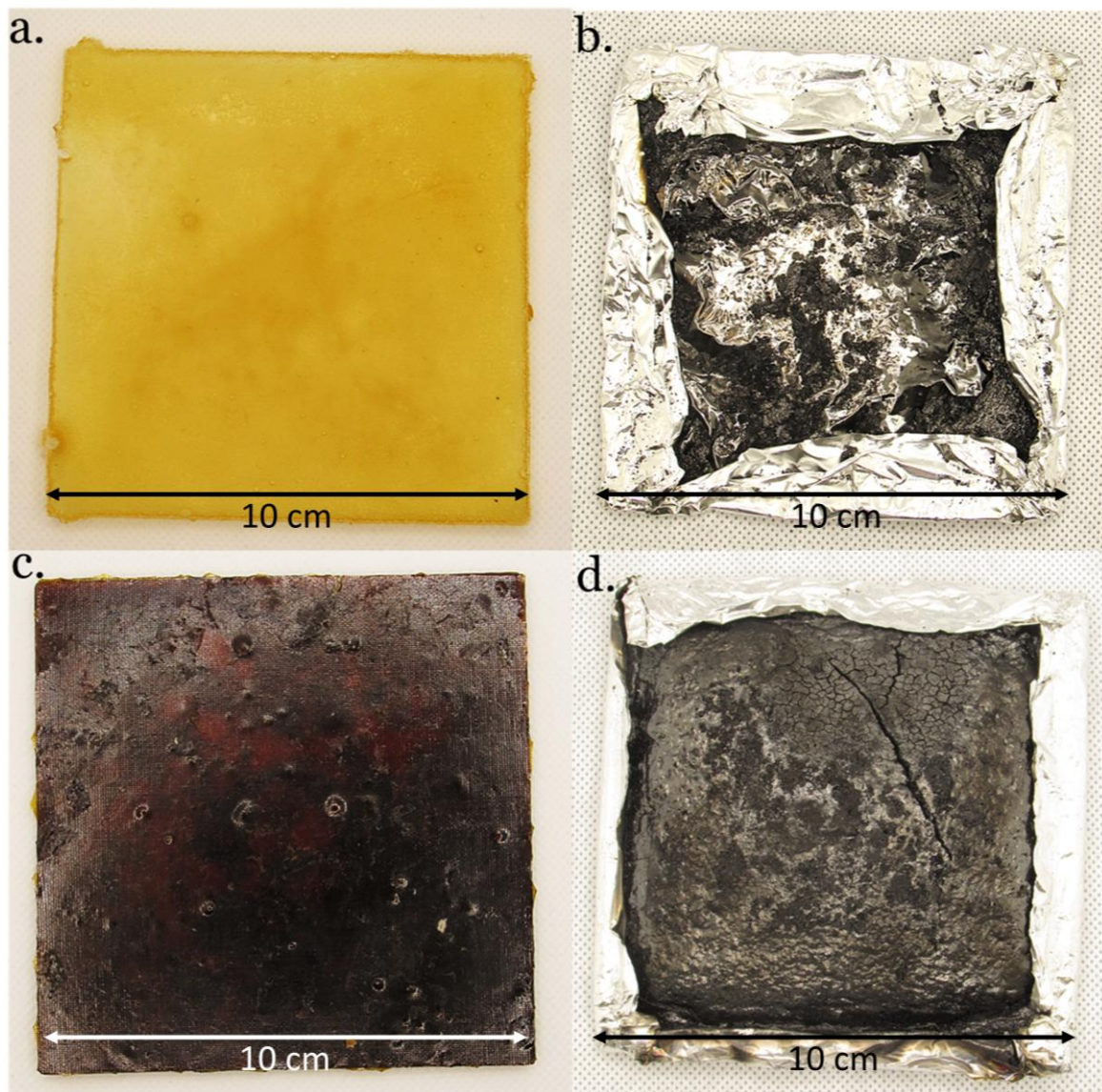
Figure 7. DGEVACE (reference) a. before and b. after cone calorimeter analysis, and DGEVAPE (vitriimer) c. before and d. after cone calorimeter analysis.
